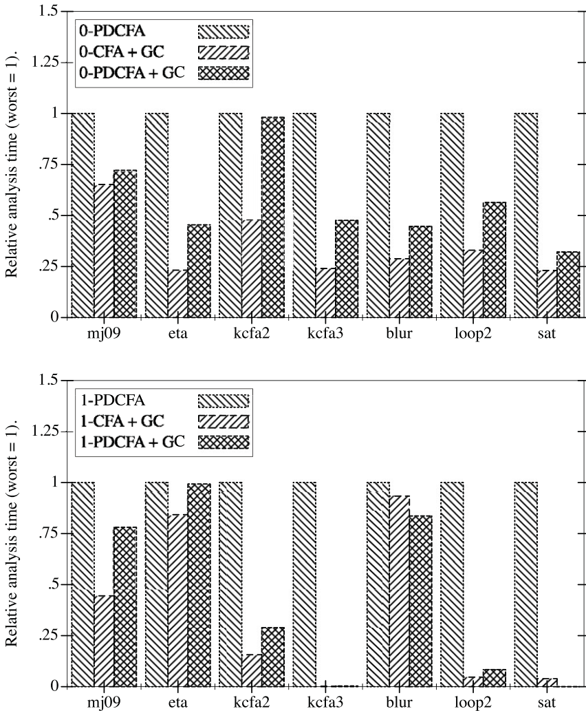
Fig. 10. Analysis times relative to worst (=1) in class; smaller is better. At the top is the monovariant OCFA class of analyses, at the bottom is the polyvariant ICFA class of analyses. (Non-GC k -CFA omitted.)
