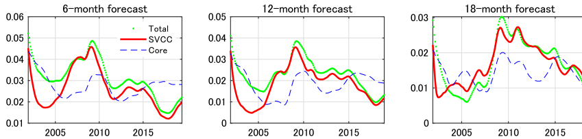
Figure 2. Forecast performance.
