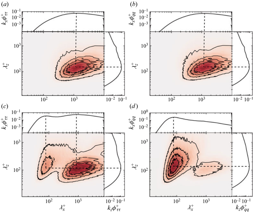
Figure 7. Two-dimensional pre-multiplied wavenumber spectra k_x k_z \Phi^+(\lambda_x^+, \lambda_z^+) with integrated one-dimensional pre-multiplied wavenumber spectra k_x \phi^+(\lambda_x^+) (top) and k_z \phi^+(\lambda_z^+) (right) of (a,c) \tau_w' and (b,d) q_w' for (a,b) M2T05 and (c,d) M8T05. The dashed lines correspond to the peak values in the one-dimensional spectra.
