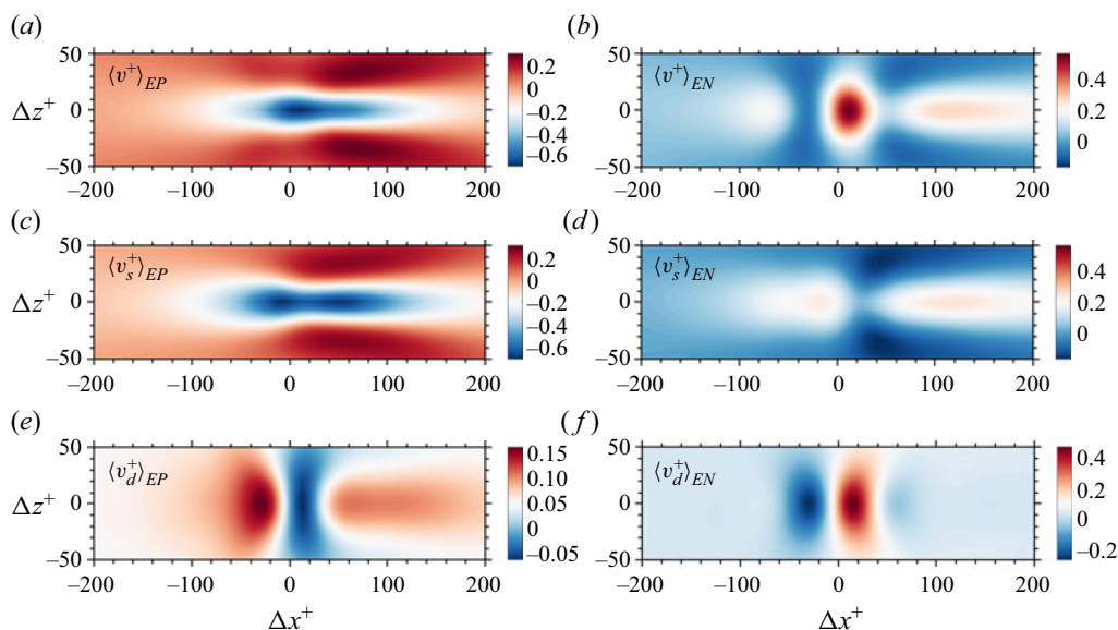
Figure 12. Contours of the conditionally averaged field based on extreme \tau'_w events for M8T05 at the y^+ = 15 plane: (a,b) the wall-normal velocity v ; (c,d) the solenoidal component v_s ; (e,f) the dilatational component v_d . Panels (a,c,e) and (b,d,f) are for EP and EN events, respectively.
