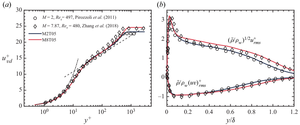
Figure 2. Statistical properties: (a) van Driest transformed mean velocity u_{vd}^+ ; (b) density-scaled turbulent intensity and Reynolds shear stress. - - - -, wall law u_{vd}^+ = y^+ ; - - - -, log law u_{vd}^+ = \log(y^+)/k + C with k = 0.41, C = 5.2 .
