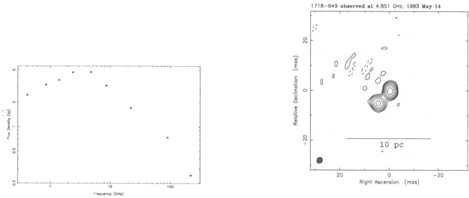
Figure 1. LHS: The total power spectrum of PKS 1718–649 between .408 and 230 GHz. The 2.3, 4.8, and 8.4 GHz points with 10% error bars are measurements from VLBI images. RHS: VLBI image of PKS 1718–649 at 4.8 GHz. The peak flux density is 2.0 \text{ Jy.beam}^{-1} and the contours are at -1, 1, 2, 4, 8, 16, 32, 64% (Beam FWHM 2.6 \times 2.3 \text{ mas} , PA = -29.5^\circ ).
