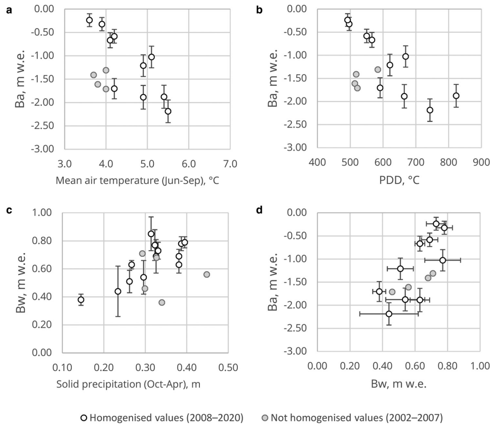
Figure 5. Relationship between meteorological parameters measured at the Barentsburg weather station (2002–20) and mass-balance values of Aldegondabreen (a, b, c) and between winter and annual mass balance of Aldegondabreen (d).
