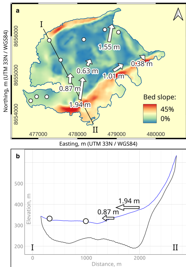
Figure 4. (a) Surface glacier velocity measured on Aldegondabreen at the ablation stakes in August 2018–August 2019 and the glacier bed slope (derived from Borisik and others, 2021); and (b) Aldegondabreen cross section and the surface velocities.
