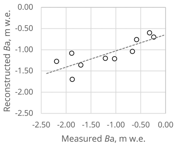
Figure 6. Scatterplot for measured and reconstructed annual mass-balance values for Aldegondabreen in 2007/08–2019/20.
