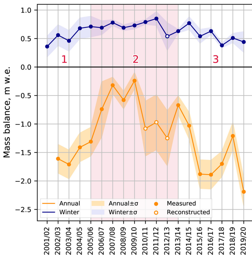
Figure 7. Annual and winter mass-balance values for Aldegondabreen in 2001/02–2019/20. The numbers 1, 2 and 3 stand for three periods of different atmospheric circulation patterns.
