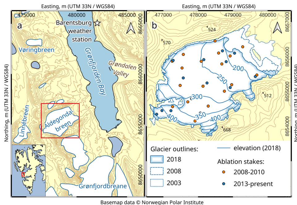
Figure 1. (a) Location of Aldegondabreen, and (b) changes in its outlines during the monitoring period and ablation stakes networks.
