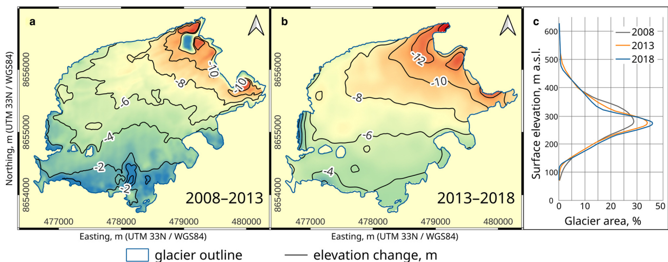
Figure 3. Elevation changes of Aldegondabreen in 2008–13 (a) and 2013–18 (b), and decadal changes in the area–altitude distribution (c).
