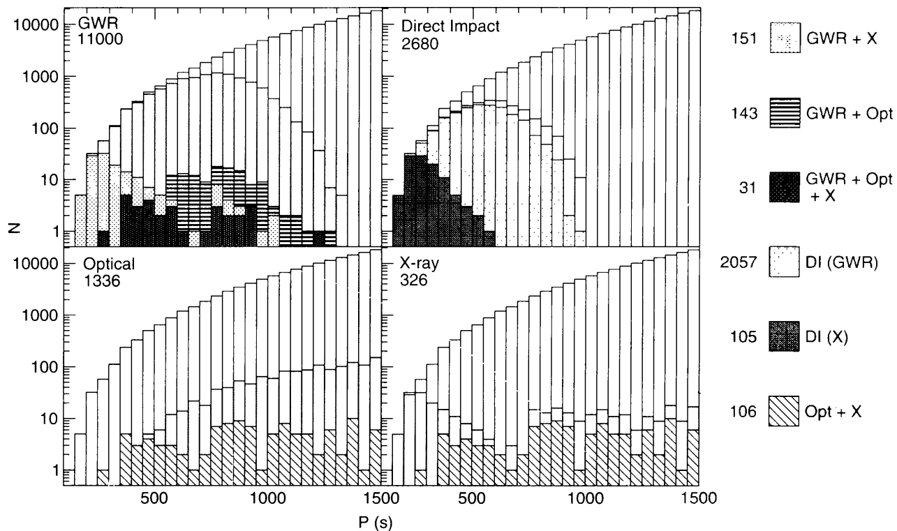
Fig. 2. Short-period AM CVn systems, subdivided in different types. Each panel shows the total population as the white histogram. The top left panel shows the systems that can be resolved by LISA in grey and they are subdivided in the ones that have optical counterparts (GWR + Opt), X-ray counterparts (GWR + X) and both (GWR + Opt + X). The top right panel shows the systems that are in the direct impact phase of accretion in grey and it is subdivided in GWR and X-ray sources. The bottom two panels show (again in grey) the populations that are detectable in the optical band (left panel) and the X-ray band (right panel). The distribution of sources detectable both in optical and X-ray bands is shown as hatched bins in both lower panels (Opt + X).
