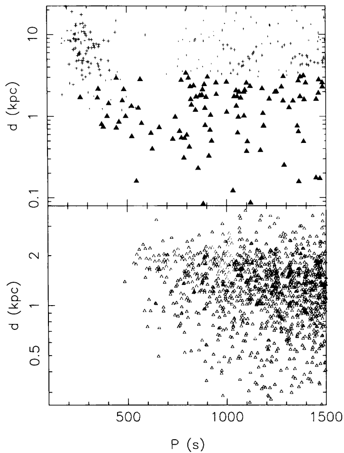
Fig. 1. Top panel: Period vs. distance distribution of systems detectable only in X-rays (pluses), and systems that are detectable in the optical and X-ray band (filled triangles). Bottom panel: Systems only detectable in the optical band.
