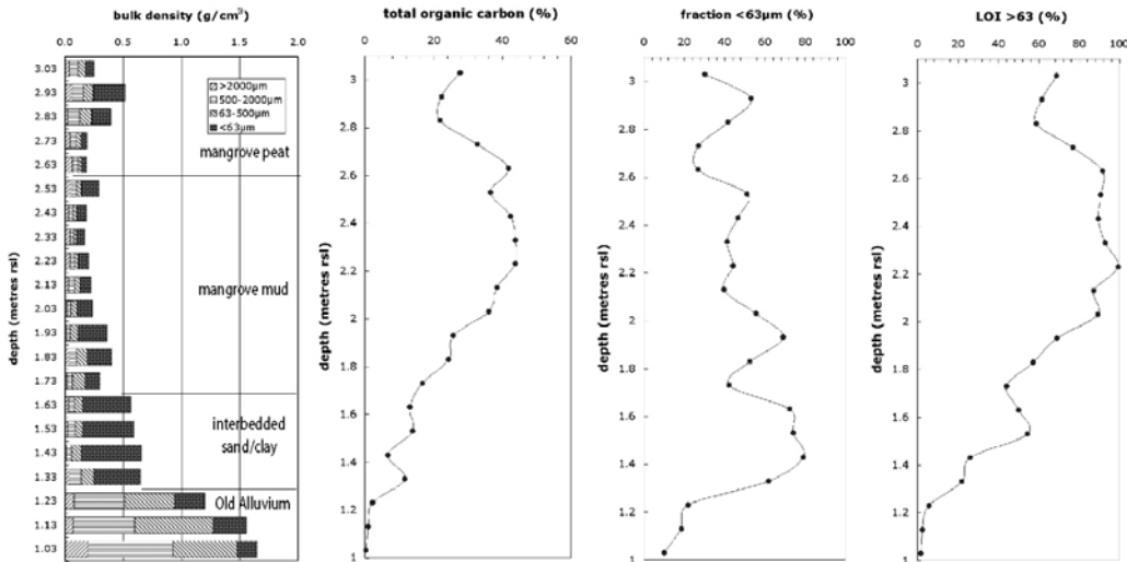
Figure 4 Contributions of different size fractions to the observed bulk density of MAR-5. Also shown are variations in F_{<63\mu m} , TOC, and LOI_{>63\mu m} through the sequence.
