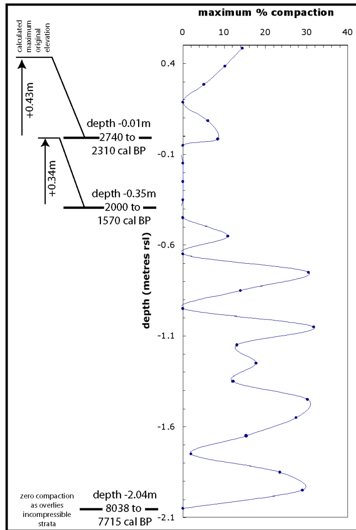
Figure 10 Percent compaction calculated for each 10-cm interval of LCK-4. Also shown is the effect of “decompacting” the sediments on the elevation of samples selected for 14 C dating. The lowermost sample is immediately above incompressible basement, and, hence, cannot be lowered by compaction (errors same as for Figure 8).
