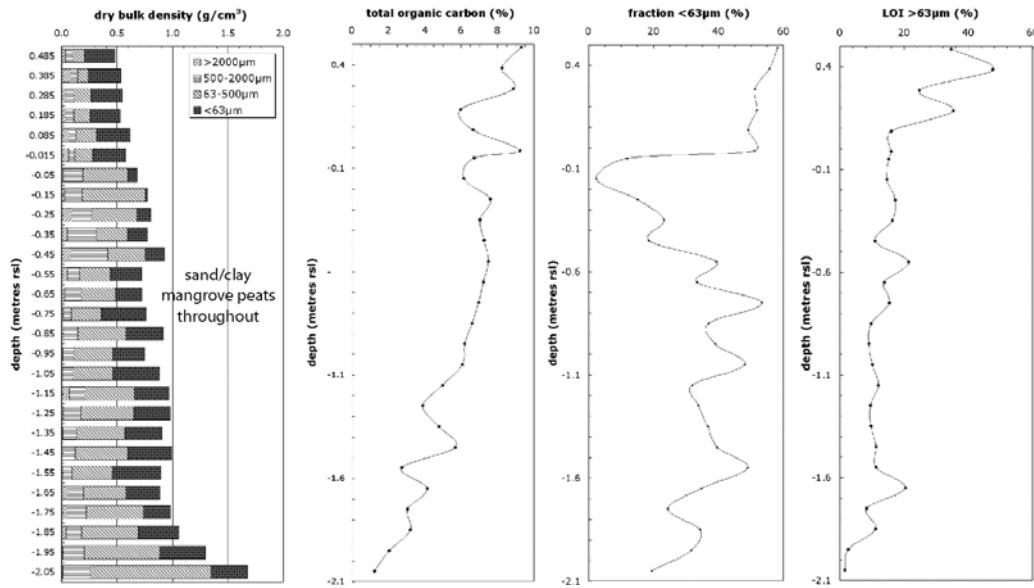
Figure 3 Contributions of different size fractions to the observed bulk density of LCK-4. Also shown are variations in F_{<63\mu m} , TOC, and LOI_{>63\mu m} through the sequence.
