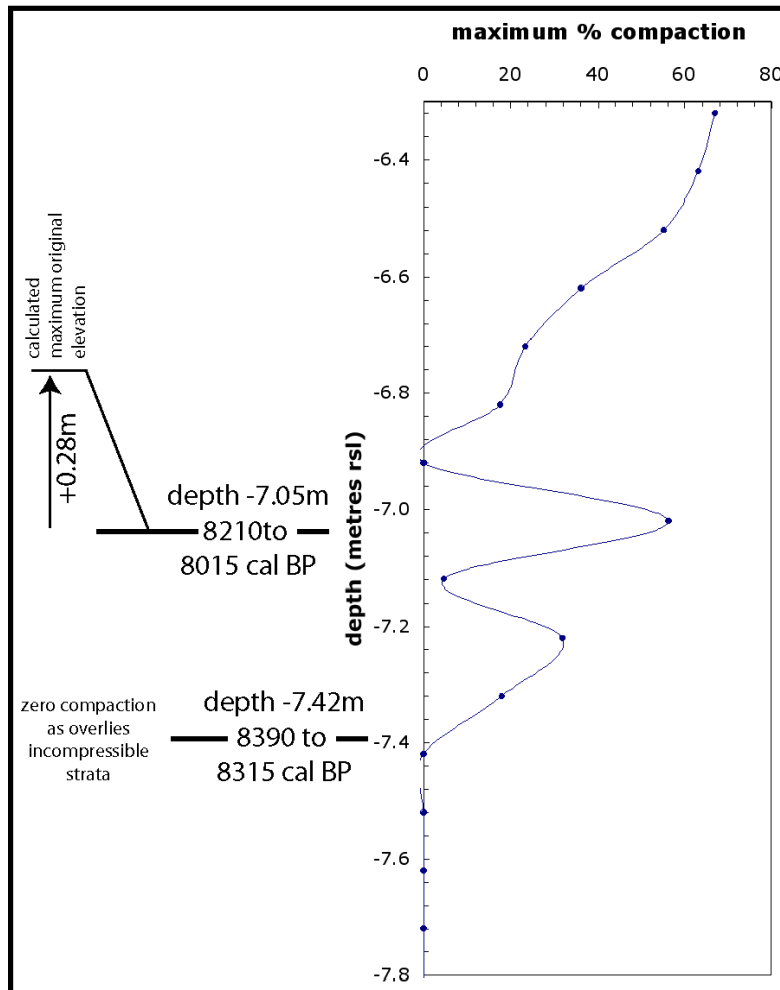
Figure 8 Percent compaction calculated for each 10-cm interval of MAR-5. Also shown is the effect of “decompacting” the sediments on the elevation of samples selected for 14 C dating. The lowermost sample is immediately above incompressible basement, and, hence, cannot be lowered by compaction. The approach used in this study yields an estimate of maximum compaction. Since the true amount of compaction is not known, the average of the values for “no compaction” and “maximum compaction” should be used for calculation of accretion rate, with the error given by half the difference between the 2 estimates.
