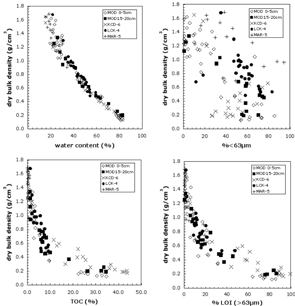
Figure 2 Relationships between DBD, F_{<63\mu\text{m}} , TOC, and \text{LOI}_{>63\mu\text{m}} for all samples analyzed in this study
