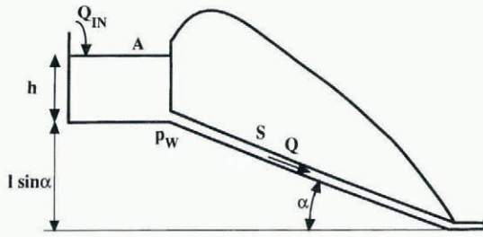
Fig. 1. Schematic cross-section of the glacier, conduit and reservoir. The symbols are defined in the Nomenclature.
