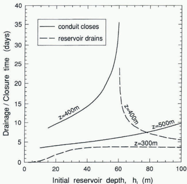
Fig. 6. Time required for the reservoir to drain, or for the conduit cross-section to decrease from 1\text{ m}^2 to 10^{-4}\text{ m}^2 , as a function of the initial reservoir depth, for three values of the glacier thickness, 300, 400 and 500 m. There is no inflow to the reservoir, Q_{IN} = 0 , and \sin \alpha = 0.1 , A = 100 h_I^2 , l = 10\text{ km} .
