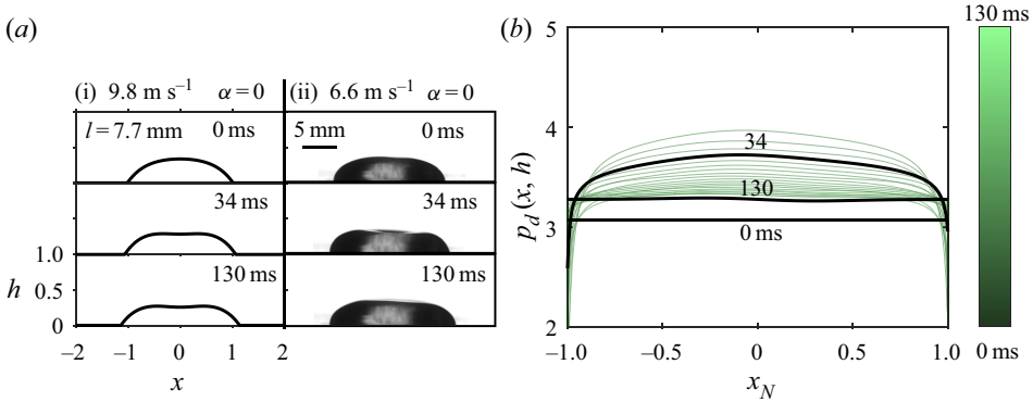
Figure 2. (a) Time-sequential images of the droplet hanging regime from the simulation and the experiment at dimensional times, t = 0, 34, 130 \text{ ms} . (i) The simulation results are for a droplet of l = 7.7 \text{ mm} under a centred jet ( \alpha = 0 ) with the jet speed U_0 = 9.8 \text{ m s}^{-1} . (ii) The experimental results correspond to l = 7.7 \text{ mm} ( 200 \mu\text{l} ), \alpha = 0 and U_0 = 6.6 \text{ m s}^{-1} . (b) We plot p_d(x, h) , the internal pressure distribution at z = h(x, t) , as a function of the normalised horizontal location, x_N = (2x - s_1 + s_2)/(s_2 + s_1) , at different time instants; p_d(x, h) corresponding to the three time instants in (i) are marked as solid black lines.
