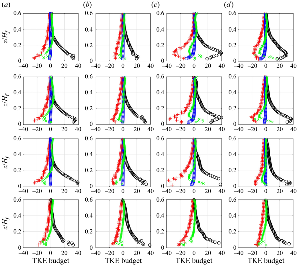
Figure 6. The TKE budget normalized by H_f/u_*^3 ; production (black, o), dissipation (red, +), turbulent diffusion (green, ×), stratification (blue, □) for dp1 ( \theta \approx 0.4 (a), \theta \approx 1.2 (b)) and dp3 ( \theta \approx 0.35 (c), \theta \approx 0.8 (d)); with increasing concentration from CW (bottom row) to saturation (top row).
