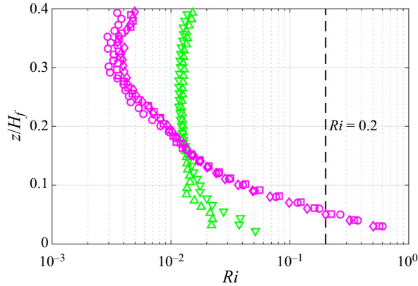
Figure 7. Comparison of flux Richardson number with the same hydrodynamic conditions with dp1 (P1S10D7_SAT (∇) and P1S10D8_SAT (Δ)) and dp3 (P3S03D9_SAT (□), P3S03D10_SAT (o) and P3S03D11_SAT (◇)); all in capacity conditions.
