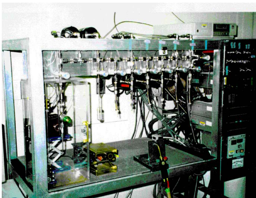
Figure 2 Photograph of the graphitization system at NIST
