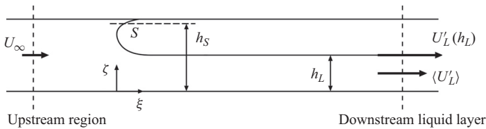
Figure 6. Shape of an elongated gas bubble in a horizontal pipe.
