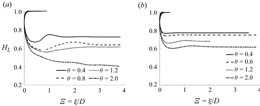
Figure 9. Profiles of elongated bubbles in viscous liquids, 0 < \mathcal{E} = \xi/D < 4 ; (a) 50 cP and (b) 200 cP.
