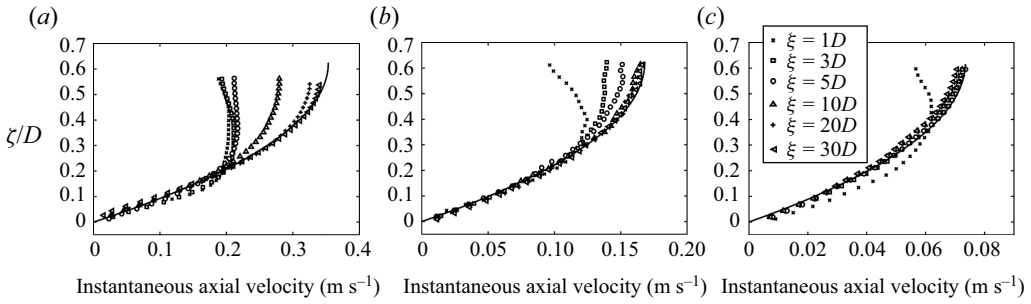
Figure 8. Vertical profiles of the axial velocity for a 1° pipe inclination at different liquid viscosities; (a) 50 cP, (b) 100 cP and (c) 200 cP.
