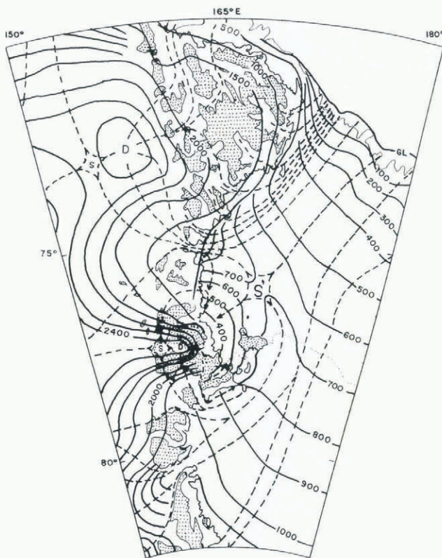
Fig. 7. LGM ice-sheet reconstruction contoured at 100 m intervals (solid lines). "GL" = grounding line; other symbols and patterns as in Figure 6. Note the similarity of ice elevations west of the Transantarctic Mountains to modern conditions. Major differences are in West Antarctica where a low-profile ice sheet occupied the entire Ross Sea. The prominent saddle north of Ross Island permitted southward ice flow into McMurdo Sound, consistent with the Stuiver and others (1981a) reconstruction. Flow from Taylor Dome (west of McMurdo Sound) was down Skelton Glacier but terminated south of Minna Bluff. Flow from Mulock Glacier rounded Minna Bluff and Ross Island before flowing south into McMurdo Sound.
