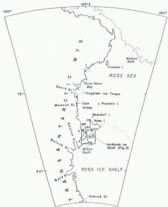
Fig. 1. Index map showing locations mentioned in text. See Figure 2 for details of the MIS. Symbols: B = Blue Glacier; CB = Cape Bird; CR = Cape Royds; F = Ferraro Glacier; K = Koettlitz Glacier; MP = Marble Point.
