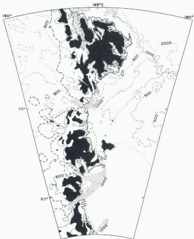
Fig. 5. Modern subglacial topography (after Drewry, 1983), contoured at 500 m intervals. Present sea level is shown by a heavy solid line where not covered by the ice sheet, and elsewhere by a heavy dashed line. Solid pattern indicates elevations above 1000 m; stippled pattern indicates depths greater than 1000 m. Note that these great depths are restricted to outlet-glacier troughs now occupied by Byrd, Mulock, David and Rennick Glaciers. Present northern margin of the Ross Ice shelf is indicated by a light dashed line.
