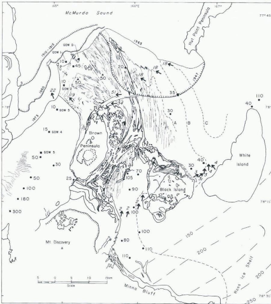
Fig. 3. McMurdo Ice Shelf thickness and ice-flow data (after Kellogg and others, 1990, fig. 17). Solid dots and arrows are thickness (in m) and velocity ( \text{m year}^{-1} ) measurements (Swithinbank, 1970), respectively; solid squares are drillholes (Gow and Epstein, 1972), except 45 m ice depth near the easternmost Dailey Islands which was extrapolated by Zolotov and Gow (1967); solid triangles are thicknesses rounded to the nearest 5 m from seismic soundings (Cook, 1963); 35 m depth is from a drillhole through the ice shelf (Paige, 1968). Dashed contour lines north of Minna Bluff are ice thicknesses (U.S. Geological Survey, 1972). Dashed lines labeled "A", "B" and "C" are from Swithinbank (1970). "A" marks the boundary between rough ice with melt streams and considerable relief (in the west) and much smoother bare ice. "B" approximates the surface equilibrium line and is extended into the Minna Bluff area based on our observations. See Swithinbank (1970) for significance of "C". Additional thickness and velocity data for the eastern part of the MIS (accumulation area) have been given by McCrae (1984). Ice-frontal position in 1947 is probably incorrect as explained by Kellogg and others (1990). Dashed lines on Brown Peninsula, Mount Discovery and Black Island are maximum extent of Ross Sea Drift (Stuiver and others, 1981a).
