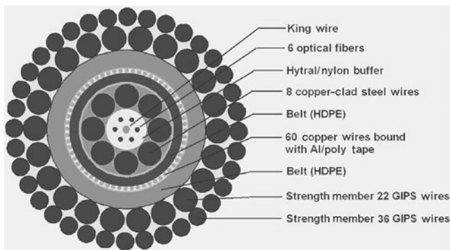
Fig. 1. Cable cross-section as designed.
