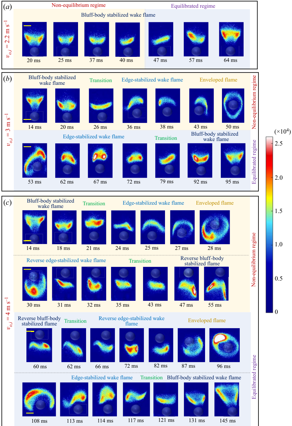
Figure 2. Time series of the flame imaging of a freely falling droplet interacting with a co-flow of velocity (a) v_{o,i} \sim 2.2 \text{ m s}^{-1} ( \tilde{v}_{o,i} \sim 3.5 ), (b) v_{o,i} \sim 3 \text{ m s}^{-1} ( \tilde{v}_{o,i} \sim 4.8 ), (c) v_{o,i} \sim 4 \text{ m s}^{-1} ( \tilde{v}_{o,i} \sim 6.3 ). A colour bar is given on the right side for the corresponding flame luminosity shown in the flame images. The different flame shapes are indicated corresponding to the flame images.
