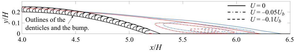
Figure 5. Mean separation region: blue, smooth case; red, denticle case. The outlines of the denticles and the bump are shown by the solid black lines for reference. The bump in the smooth case aligns with the envelope of the crown in the denticle case.
