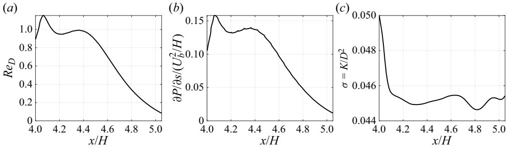
Figure 15. Profiles of the pore flow Reynolds number, pressure gradient and the non-dimensional Darcy permeability in case DT. Measured at 25% \delta_h and moving averaged over a window of the streamwise spacing between denticles.
