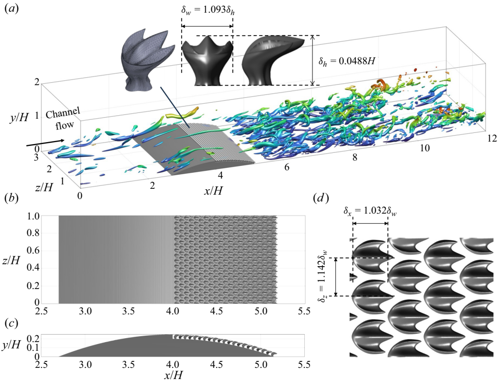
Figure 2. (a) Computational configuration. An instantaneous flow field of case DT is shown, visualized by the isosurfaces of the second invariant of the velocity-gradient tensor and coloured by the distance from the bottom wall. Inset, three-dimensional (3-D) model of the shark denticle (Wen et al. 2014). (b–d) Top and side views of the bump and denticle array.
