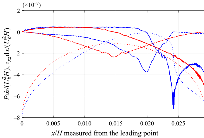
Figure 17. Profiles of the normal and shear forces on the surface of the 2-D structure in the Darcy pore flow simulations: blue, denticle neck at 25% \delta_h ; red, circle of the same cross-sectional area as the denticle neck at 25% \delta_h . Here, — Pdz , — 1/Re\partial U/\partial z dx , ... structure outline for location reference. Each profile is plotted from the leading point to the end of the corresponding structure. The pressure at the leading point is set to zero.
