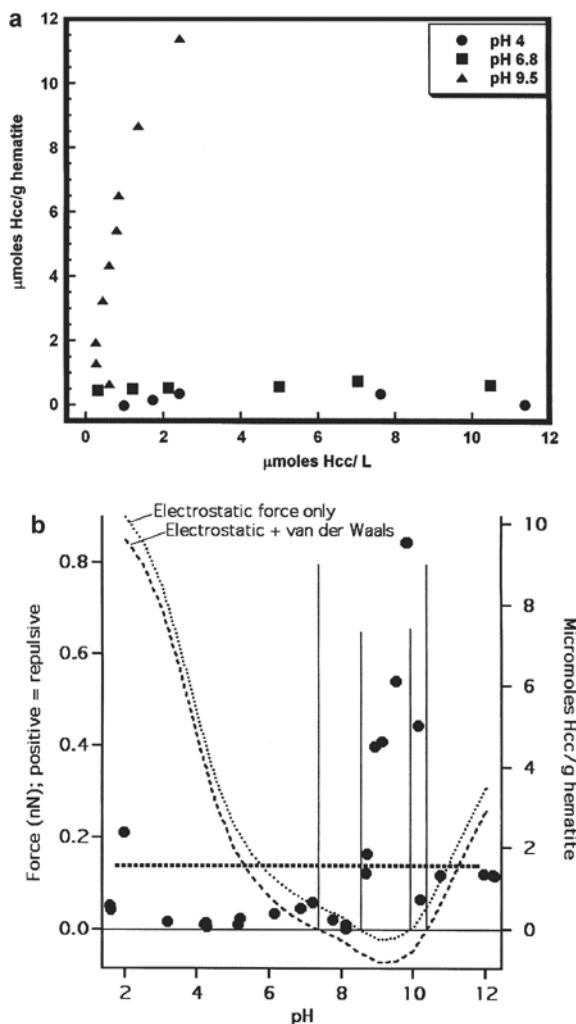
Figure 1. (a) Sorption isotherms of \mu moles of Hcc sorbed/g of hematite vs. \mu moles of dissolved Hcc/L of supernatant solution at pH 4.0 \pm 0.05 , 6.83 \pm 0.07 , and 9.5 \pm 0.10 . (b) Sorption of Hcc on hematite as a function of pH (filled circles, right-hand axis). Black dotted and dashed curves give overall repulsive (positive) or attractive (negative) forces between hematite and Hcc (references for Hcc isoelectric point and hematite point of zero charge are given in the text; Hamaker constant for van der Waals calculation from Schudel et al. (1997) and Neal et al. (1999)). The thick dashed horizontal line gives the amount of sorption corresponding to one monolayer of Hcc on hematite in hexagonal close packing. The vertical lines show the zero crossing points for the force calculations with and without van der Waals forces for easier comparison to the sorption data.
