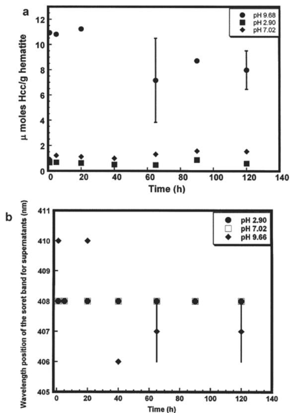
Figure 3. (a) Sorption kinetics for Hcc sorbing on hematite over a period of 1–120 h for \text{pH} 2.9 , 7.0 and 9.7; (b) wavelength position of Soret bands in supernatant solutions from sorption experiments as a function of time at \text{pH} 2.9 , 7.0 and 9.7.
