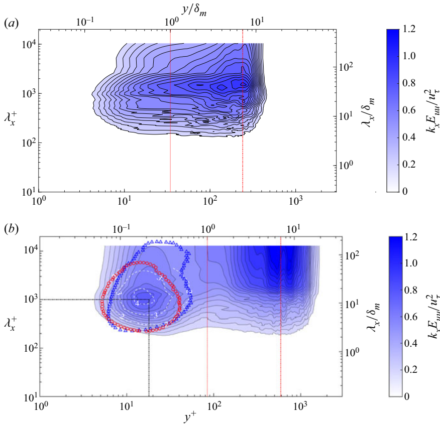
Figure 6. Normalised premultiplied spectra contours of streamwise fluctuation k_x E_{uu}/u_\tau^2 for the turbulent NCBL (DNS-D) in (a) the ‘classical’ regime, Gr_\delta = 1.1 \times 10^6 ( Re_\tau \approx 34 ), and (b) the fully turbulent ultimate regime, Gr_\delta = 2.7 \times 10^7 ( Re_\tau \approx 85 ). Black dash-dotted lines indicate the inner energy peak site at \lambda_x^+ \approx 1000 and y^+ = 18 ; the red dotted line is at the velocity maximum location y/\delta_m = 1 , which differentiates the near-wall region and the outer bulk flow; the red dash-dotted line indicates the outer energy peak site at y/\delta_m \approx 7 . White dashed lines indicate contour levels k_x E_{uu}/u_\tau^2 = 2, 3, 4 in the near-wall region for DNS-A (Ke et al. 2020) at Gr_\delta = 7.7 \times 10^7 . Red circles indicate the near-wall site contour level k_x E_{uu}/u_\tau^2 = 1.2 for a turbulent channel flow at Re_\tau = 935 (Del Alamo et al. 2004); blue triangles indicate the near-wall site contour level k_x E_{uu}/u_\tau^2 = 1.2 for a turbulent boundary layer at Re_\tau = 7300 (Hutchins & Marusic 2007b).
