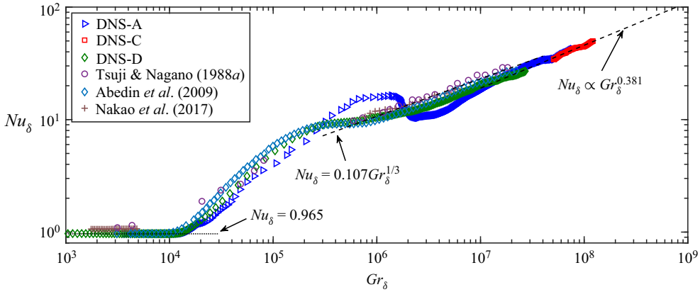
Figure 3. Nusselt number development of the NCBL. The black dotted line represents the laminar analytical value Nu_\delta = 0.965 (Ke et al. 2019), and the black dashed lines indicate the empirical 1/3 power law correlation for the ‘classical’ regime, and the 0.381 power law for the fully turbulent regime (Ke et al. 2021).
