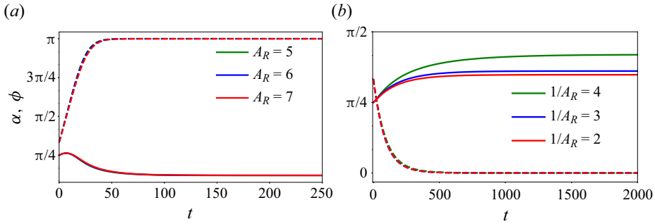
Figure 13. Orientation angles \alpha(t) and \phi(t) for (a) prolate and (b) oblate spheroids when the external force and viscosity gradient are perpendicular ( \mathbf{F} = \hat{z} , \nabla\eta = \beta\hat{x} ). The dashed curves show the evolution of \phi , while the solid curves show the evolution of \alpha . For all cases, the initial orientation is given by the ordered pair (\phi_0, \alpha_0) = (\pi/3, \pi/4) and the dimensionless viscosity gradient is \beta = 0.1 . The results show that \phi \rightarrow 0 or \pi , and hence, the particle becomes co-planar with \mathbf{F} and \nabla\eta .
