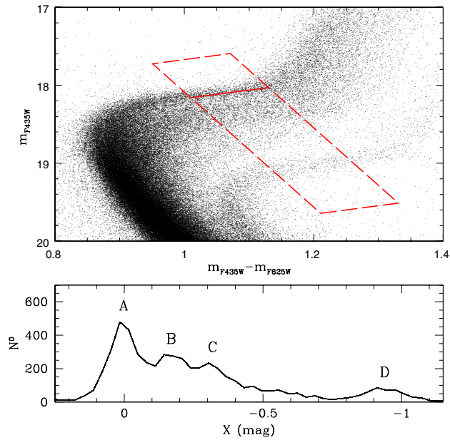
Figure 3. The multiple SGB in Omega Centauri. There are at least 4 distinct SGBs, plus a small fraction of stars spreaded between SGB-C and SGB-D (from Villanova et al. 2007).
