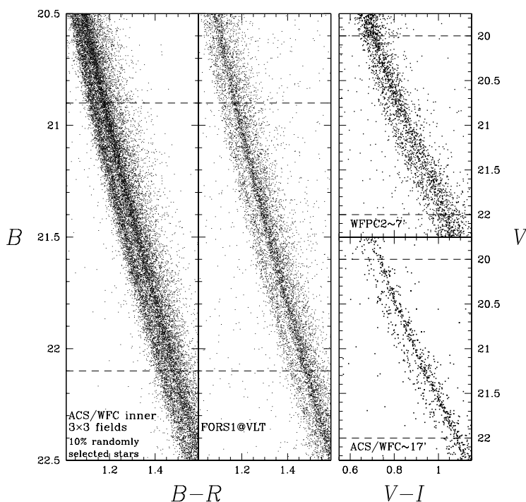
Figure 2. The double MS of Omega Centauri. The MS split is visible from the cluster center to its outskirts, though the ratio of the number of stars populating the two sequences decreases from the cluster core to its outer envelope (from Bellini et al. 2008, in preparation ).
