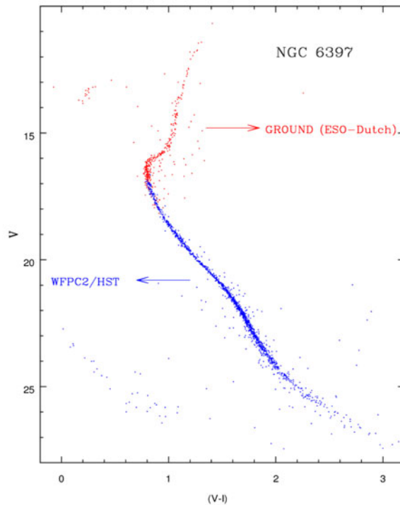
Figure 1. The CMD of NGC 6397 shows very narrow sequences and a well defined TO, supporting the idea that, in general, GCs are populated by coeval and chemically homogeneous stars.
