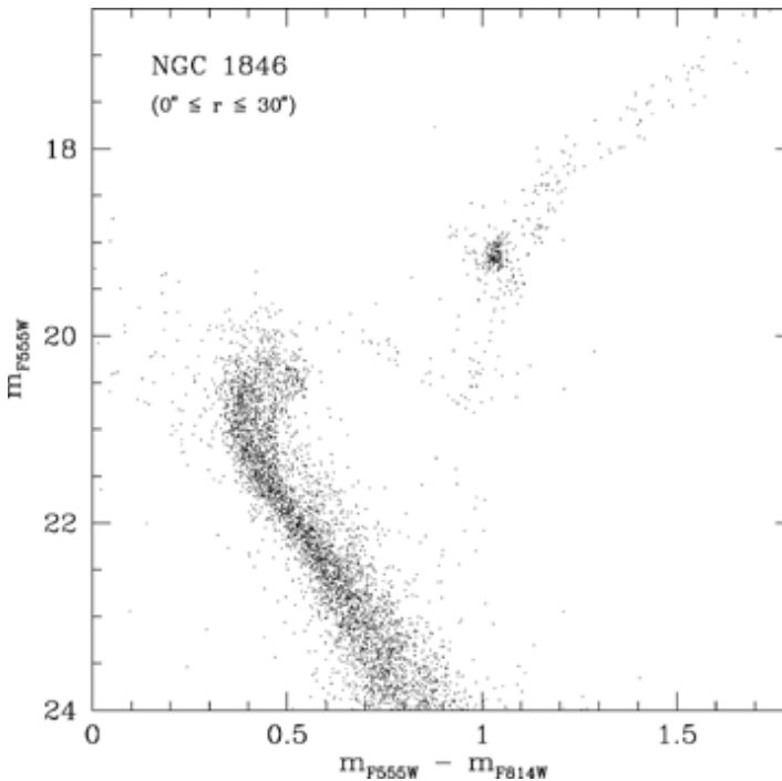
Figure 7. The double main sequence turn off of the Large Magellanic Cloud cluster NGC 1846 (from Mackey & Broby Nielsen 2007).
