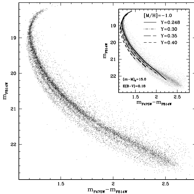
Figure 4. The spectacular triple MS of NGC 2808. Note the narrowness of the turnoff. The isochrone fitting in the inset shows that the bluest sequence can be reproduced only with a He content as high as Y = 0.40 (from Piotto et al. 2007).
