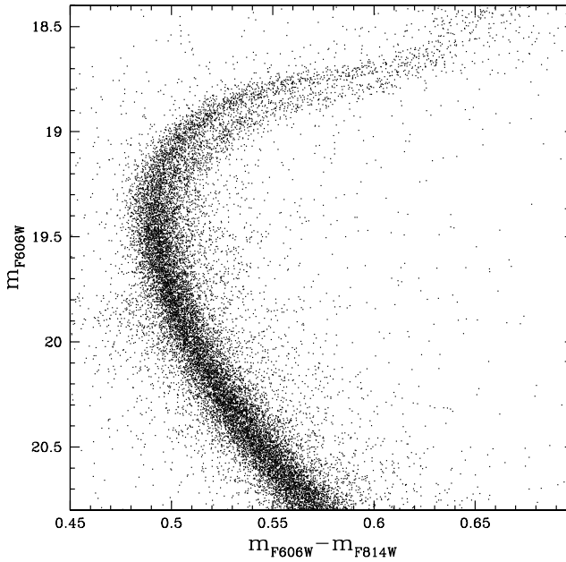
Figure 5. The double SGB in NGC 1851. The two SGBs are separated by about 0.12 magnitudes in F606W (from Milone et al. 2007)
