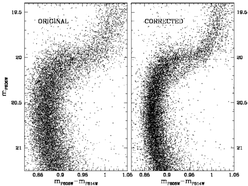
Figure 6. After the correction for differential reddening, also NGC 6388 shows a double SGB (Piotto et al. 2008, in preparation ).
