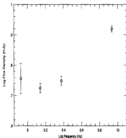
Figure 1. Radio Spectrum of GX 339-4 on 1997 Feb 18.
