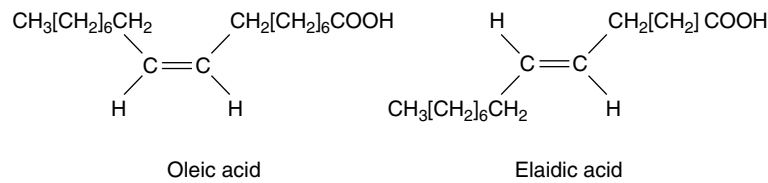
Fig. 1. Cis - and trans -MUFA: 18:1 ( n -9) cis or oleic acid, and 18:1 ( n -9) trans or elaidic acid, respectively.
