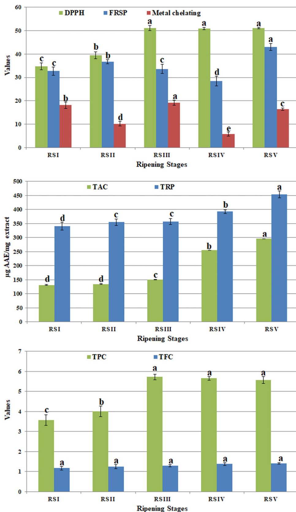
Figure 2. Total phenolic content (TPC \mu\text{g GAE}/\text{mg extract} ), total flavonoid content (TFC \mu\text{g QE}/\text{mg extract} ), antioxidative response (total antioxidant capacity (TAC \mu\text{g AAE}/\text{mg extract} ) and total reducing power (TRP \mu\text{g AAE}/\text{mg extract} )), and free radical scavenging activity (% inhibition) The values are mean of triplicates. The small alphabets on bars represent significant difference between the mean by LSD at p < 0.05 .
