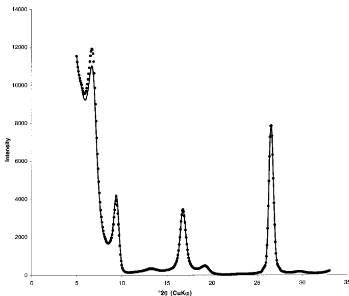
Figure 4. Comparison of LU (dots) and IU-PL (thick line) modeling for a two-component EG I-S MLM, W_1 = 0.70 , p_{SS} = 0 . The tetrahedral charge of illite comes from Si-Fe substitution ( \text{Si}_{3.6}\text{Fe}_{0.4} ).
