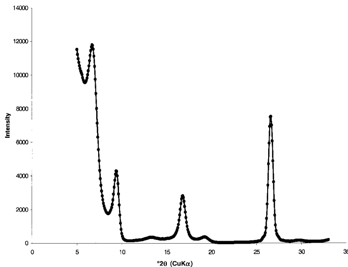
Figure 3. Comparison of LU (dots) and IU-PL (thin line) XRD modeling for a two-component EG I-S MLM, W_1 = 0.70 , p_{SS} = 0 . The tetrahedral charge of illite comes from Si-Al substitution ( \text{Si}_{3.6}\text{Al}_{0.4} ). The two intensity distributions cannot be seen on this scale.
