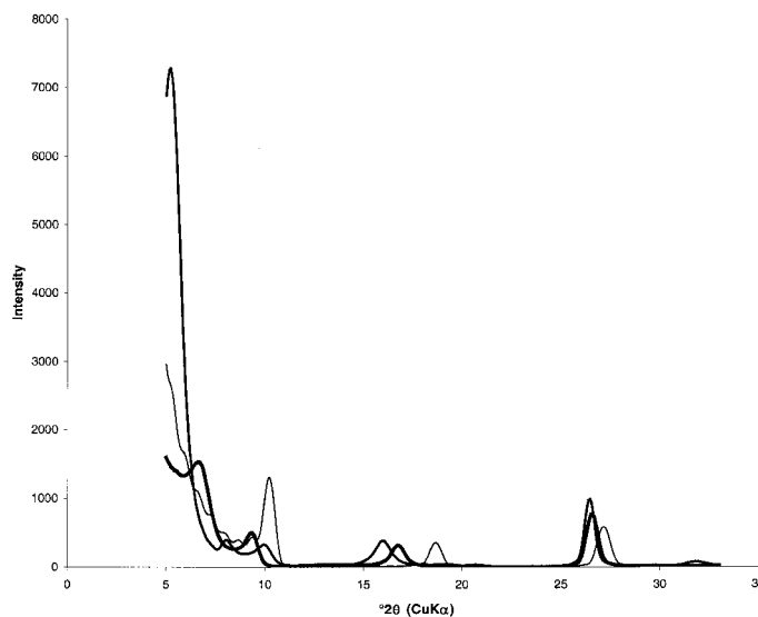
Figure 5. Comparison of IU-PL (thick line) and IU-NPL XRD models for a two-component EG I-S MLM, W_I = 0.70 , p_{SS} = 0 . For the IU-NPL models the d value of the HC-LC IUs is either the illite one (thinner line) or the smectite one (thicker line).
