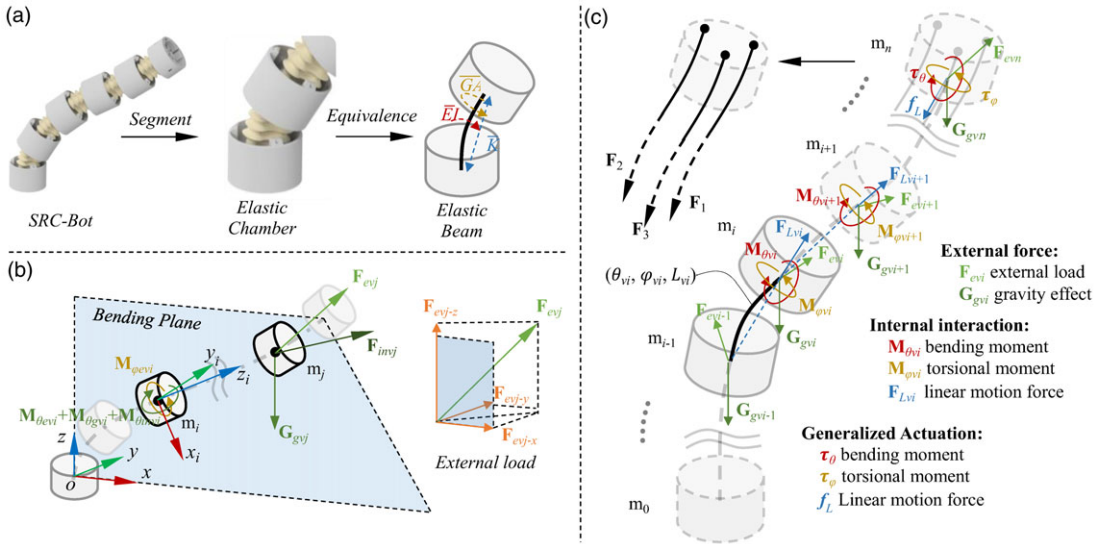
Figure 4. Structure equivalence and dynamics analysis of SRC-Bot: (a) Equivalence of the segment of SRC-Bot, where E\bar{I} is the bending stiffness, \bar{G}A is the torsional stiffness, and \bar{K} is the linear motion stiffness; (b) moment contributed by external load and gravity, where \vec{M}_{\theta_{\varphi_{evi}}} and \vec{M}_{\theta_{evi}} are the moment generated by the external force \mathbf{F}_{evj} in bending and rotation direction, respectively. \vec{M}_{\theta_{gvj}} is the moment caused by gravity, \vec{M}_{\theta_{invi}} is the moment owing to the inertia force; (c) mechanics analysis of the segment of SRC-Bot, where \mathbf{F}_i is the force actuated on cables.
