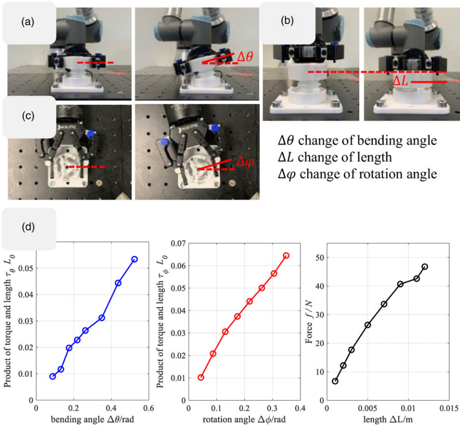
Figure 8. Equivalent stiffness identification: (a) bending stiffness; (b) linear stiffness; (c) rotation stiffness; (d) identified stiffness curves.
