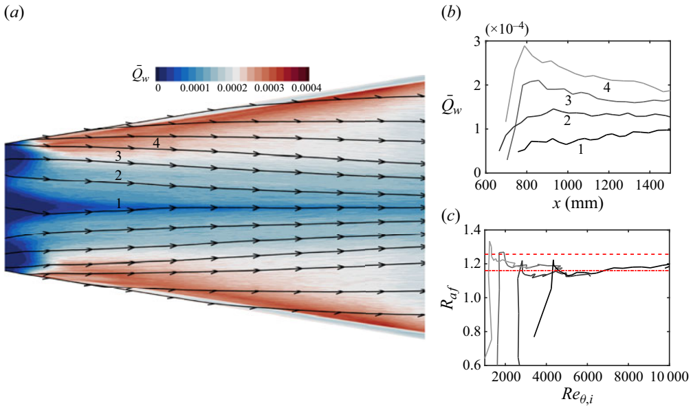
Figure 7. (a) Mean wall heat flux \bar{Q}_w (flooded contour) overlaid by the wall limiting streamlines. (b) Streamwise variations of \bar{Q}_w . (c) The Reynolds analogy factor R_{df} along the four wall limiting streamlines in (a). Dashed and dash-dotted lines represent, respectively, Pr^{-2/3} and 1.16.
