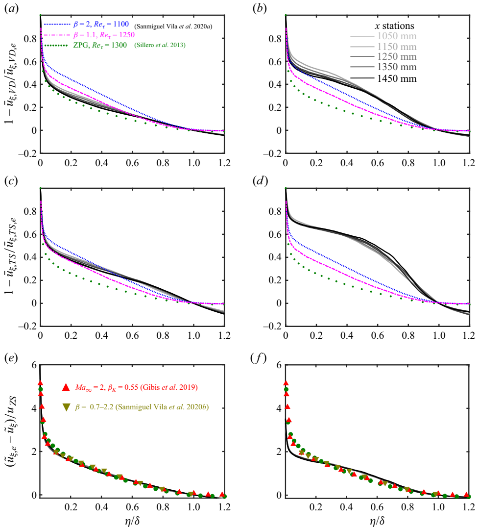
Figure 12. Mean velocity deficit profiles in meridian planes ( a,c,e ) \phi = 140^\circ and ( b,d,f ) \phi = 180^\circ expressed as ( a,b ) 1 - \tilde{u}_{\xi,VD}/\tilde{u}_{\xi,VD,e} , ( c,d ) 1 - \tilde{u}_{\xi,TS}/\tilde{u}_{\xi,TS,e} , and ( e,f ) (\tilde{u}_{\xi,e} - \tilde{u}_{\xi})/u_{ZS} , with u_{ZS} the Zagarola–Smits velocity scale.
