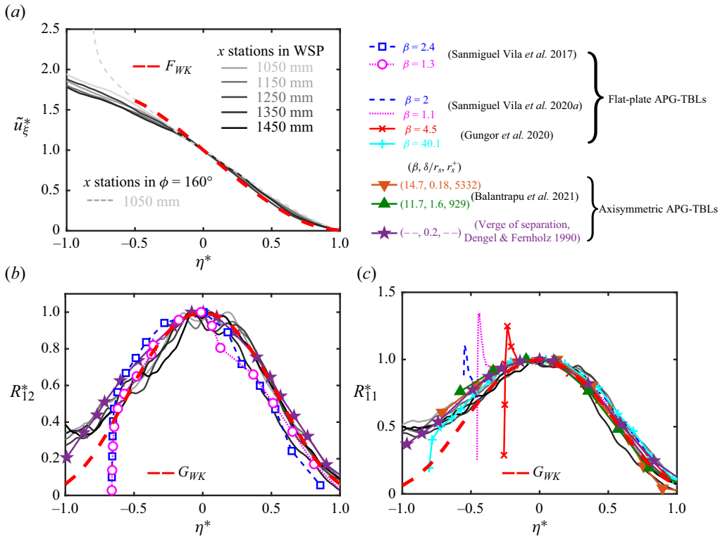
Figure 16. Wall-normal distributions of (a) velocity deficit \bar{u}_\xi^* , (b) Reynolds shear stress R_{12}^* and (c) streamwise Reynolds normal stress R_{11}^* .
