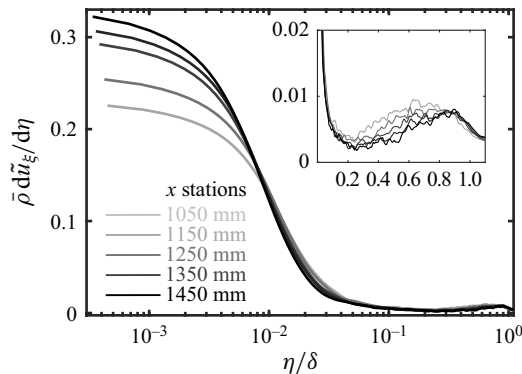
Figure 17. Mean velocity gradient \bar{\rho} d\bar{u}_\xi/d\eta in the WSP at different streamwise stations.
