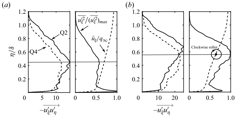
Figure 18. Wall-normal distributions of the tangential Reynolds stresses -u'_\xi u'_\eta^+ carried by ejection (Q2, u'_\xi < 0, u'_\eta > 0 ) and sweeping (Q4, u'_\xi > 0, u'_\eta < 0 ) events, the mean velocity \bar{u}_\xi / q_\infty and the normalized streamwise velocity fluctuation intensity u'^2_\xi / (u'^2_\xi)_{max} in meridian planes (a) \phi = 160^\circ and (b) \phi = 180^\circ at x = 1050 mm.
