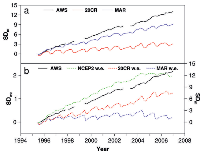
Fig. 5. (a) SD_m from the AWS (black), 20CR (red) and MAR (purple) and (b) SD_{we} from NCEP2 (dashed green), 20CR (dashed red) and MAR (dashed purple) for the CP site.
