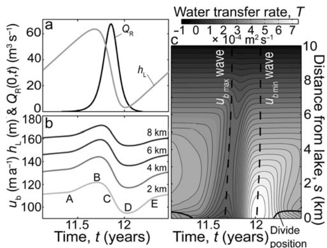
Fig. 3. Evolution of (a) lake level, h_L(t) , and channel discharge at the lake, Q_R(0, t) ; (b) sliding velocity, u_b(s, t) ; and (c) cavity-channel water transfer rate, T(s, t) in the limit cycle indicated by the boxes in Figure 2g and h. M_C = 1 \times 10^{-3} \text{ m}^2 \text{ s}^{-1} , R_k = 1 .
