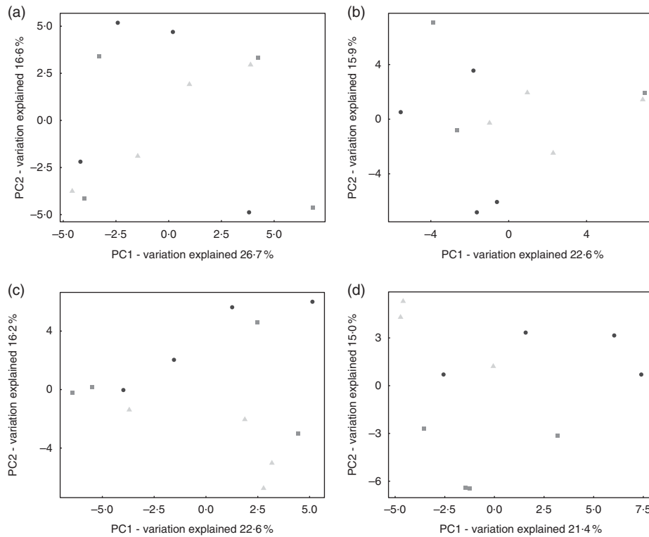
Fig. 2. Principal component analysis of square root transformed Operational Taxonomical Units (OTU) abundances in faecal samples ( n = 46 ) collected at (a) 23, (b) 25, (c) 27 and (d) 30 d of age displaying principal components (PC)1 and 2. Points are coloured according to diet. ●, Colostrum; ▲, milk replacer; ■, sow milk.
