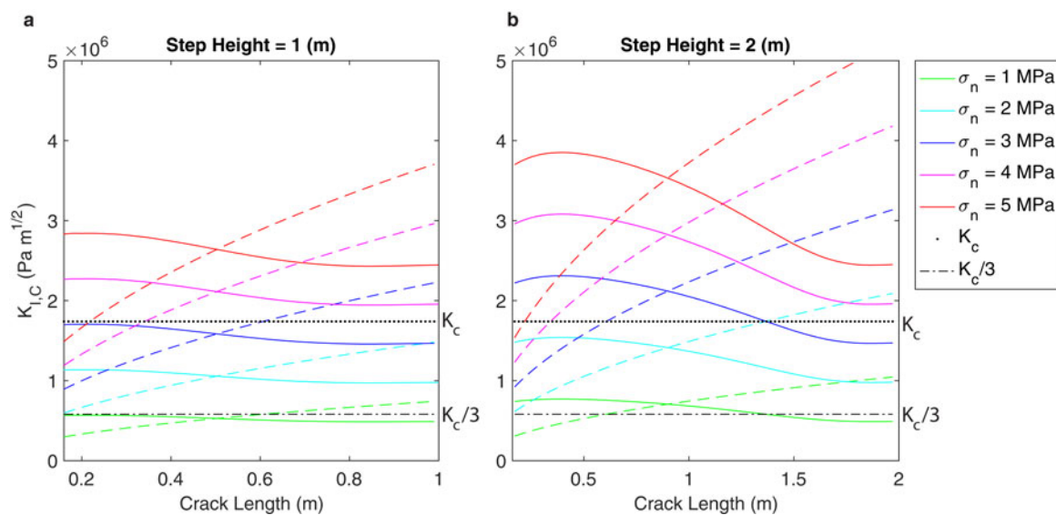
Fig. 4. Stress intensity ( K_I ) values for FEM simulations with step heights of 1 and 2 m. Solid lines show K_I values from the FEM simulations at variable applied normal stresses ( \sigma_n ) on the top of the block. Dashed lines are the values based on Eqn 2 and the correction factor 0.66 used by Hallet (1996) to convert applied normal stresses to far-field tensile stresses. The dotted line is the fracture toughness ( K_c ) value for Balmholtz limestone. The dot-dashed line is the threshold for subcritical crack growth ( K_c/3 ).
