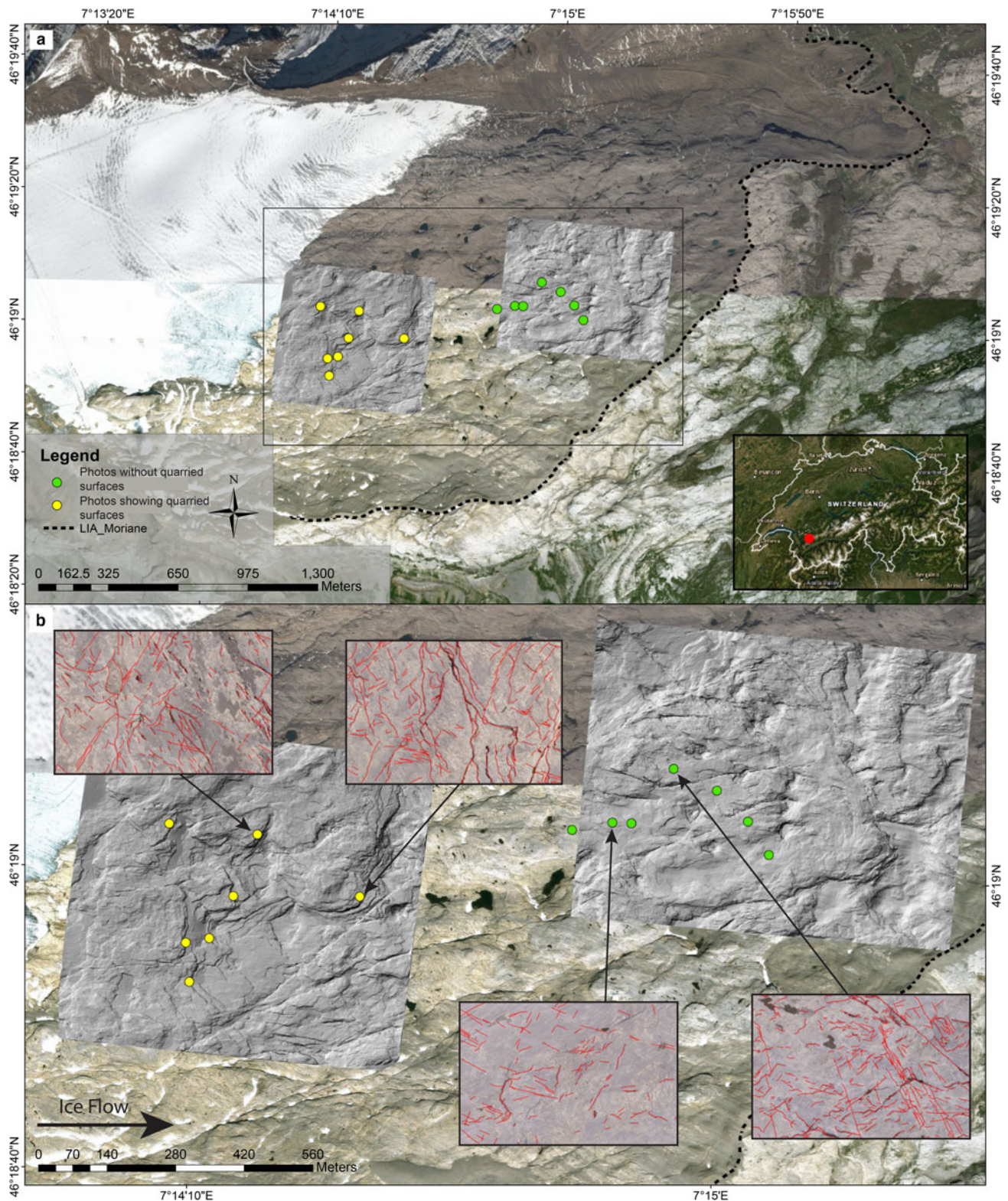
Fig. 1. DEMs with hillshading of the Tsanfleuron forefield overlain on 2012 and 2016 DigitalGlobe satellite imagery. Locations of photos with quarried surfaces (yellow dots) and without quarried surfaces (green dots), which were used for the fracture analysis, are also plotted. (a) Broad view of the forefield with the outer limit of the LIA moraine outlined with a black dashed line. The black box shows the location of (b). (b) Expanded portion of the forefield with inset photos that show examples of traced discontinuities in four photos.
