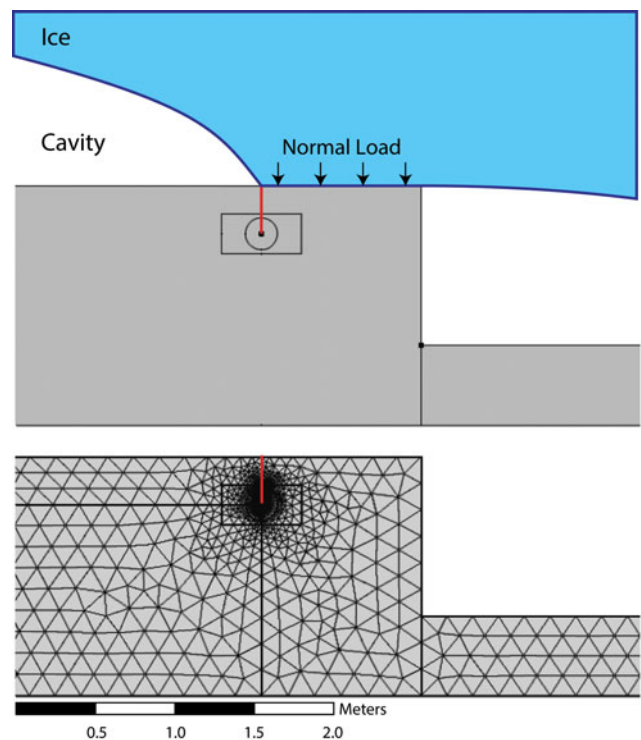
Fig. 2. FEM geometry and mesh used in the fracture-growth simulations. The red line shows the location of the fracture. The circle and rectangle around the crack tip are the paths of integration ( \Gamma ) used to calculate the J -integral. Water pressure in cavities is assumed to be zero to maximize the deviatoric stresses on the crack.
