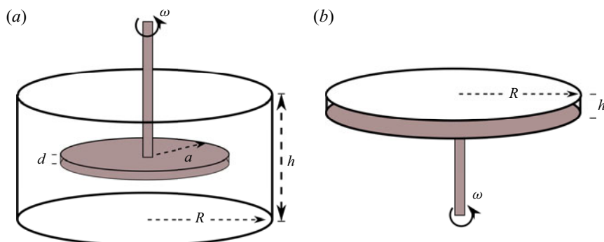
Figure 1. Rotational flows in a cylindrical cavity, radius R and height h . (a) Sketch of a typical rotating-disk experiment. The disk, radius a and thickness d , is usually placed halfway between the bottom of the container and the free surface of the fluid. Mass transfer takes place on the bottom surface of the disk, while the remaining surfaces are passivated. The outer cylinder in the simulations is larger than indicated in the sketch, R = 2h = 4a . (b) Sketch of a rotor–stator geometry. The lower disk (shaded) rotates with an angular velocity \omega , while the upper disk and sidewalls are stationary; R = 5h .
