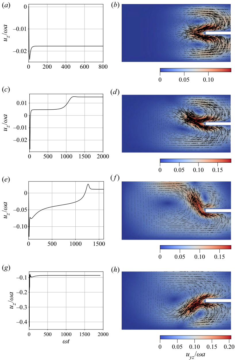
Figure 7. Time-independent flows around a rotating disk. Time traces of the axial velocity at r = 1.5a , z = 0.25h (and elsewhere) show that the velocity field is time invariant after an initial transient. Maps of the steady flow in the plane x = 0 are shown in panels (b,d,f,h). Panels (a–d) have no-slip boundaries on all surfaces: (a,b) Re = 50 ; (c,d) Re = 100 . Panels (e–h) include a free-surface boundary condition at z = h : (e,f) Re = 100 ; (g,h) Re = 120 . Arrows represent the magnitude and direction of the flow within the yz plane. The colour scale indicates the magnitude of the in-plane velocity field, u_{yz} = (u_y^2 + u_z^2)^{1/2} .
