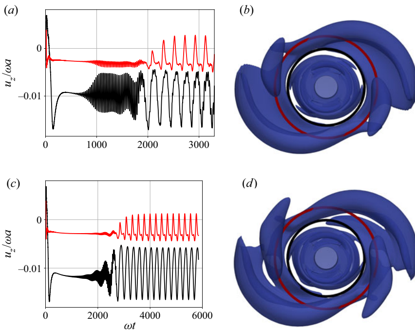
Figure 15. Oscillatory flow at Re = 900 and Re = 1000 . (a) Axial velocity at Re = 900 , (b) isosurface at Re = 900 , (c) axial velocity at Re = 1000 and (d) isosurface at Re = 1000 . The probe locations are at r = 1.5a , z = 0.25h and r = 2a , z = 0.45h ; the isosurface contour is Q = 0.0032\omega^2 . The probes lie on the circles of the same colour.
