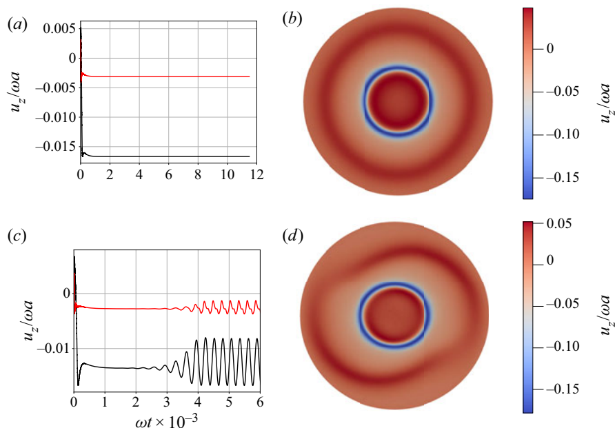
Figure 8. Onset of instability between Re = 600 and Re = 800 . Axial velocity measured by probes located at r = 1.5a, z = 0.25h (black) and r = 2a, z = 0.25h (red), together with colour contours of the axial velocity in the plane z = 0.125h : (a,b) Re = 600 and (c,d) Re = 800 .
