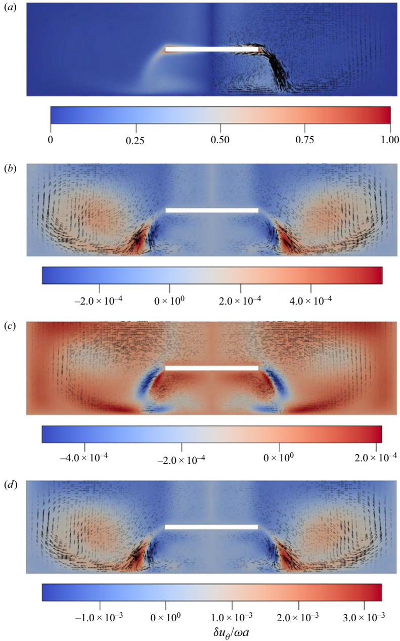
Figure 12. Maps of the mean flow (a), and perturbation \delta \mathbf{u} at \omega t = 5960 (b,c). Slice (c) is rotated by +45^\circ with respect to (b). Panel (d) is delayed by seven complete oscillations from panel (b); the length of the lines and the colour scale have been adjusted for the growth of the eigenmode, a factor of 5.55 over this time interval. Flow in the plane \delta u_r, \delta u_z is indicated by arrows, while the perpendicular flow \delta u_\theta is indicated by the colour scale. The arrows indicating the direction of the flow have been clipped from the left side of panel (a) so the variations in colour are more visible.
