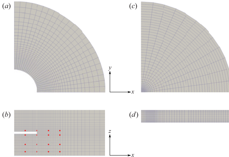
Figure 2. Finite-volume mesh for rotating disks. (a) The central layer of a rotating disk geometry, showing the area excluded by the disk. The mesh is created in four quadrants of which only one is shown. (b) Side view of the fluid domain (grey) and rotating disk (white). The radius of the fluid cell R = 4a , the height h = 2a and the thickness of the disk d = 0.1a . The origin z = 0 is on the base of the container, and the disk is centred at (0, 0, h/2) . The mesh lines are graded in the vicinity of the disk to improve resolution. The upper and lower layers of the disk are fluid filled and the quadrants are connected by a central square of length a . The red squares indicate the probe locations discussed in § 4.3.2: the radial positions are r = 0.5a, a, 1.5a, 2a , and the axial positions are z = 0.1h, 0.25h, 0.45h, 0.55h . (c) Top view of the rotor–stator geometry. The cavity is meshed using a central square (length 0.035R ), with the small cells near the centre growing larger. (d) Side view: the mesh lines are graded near the rotor and stator plates.
