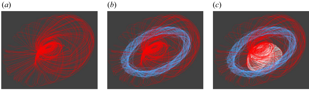
Figure 10. Streamlines of the mean flow \bar{u}(r, z) at Re = 700 . The tracers within each circulation zone are indicated by a different colour: (a) red, zone 1 recirculation; (b) blue, zone 2 vortex roll; (c) white, zone 3 vortex roll underneath the disk.
