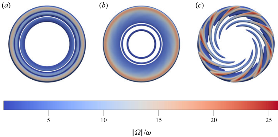
Figure 5. Isosurface of Q = 0.19\omega^2 (3.2), showing circular and spiral vortices in the stator layer, at a time of (a) \omega t = 25 , (b) \omega t = 60 and (c) \omega t = 250 ; the mesh resolution is \mathcal{R}_{442} . The top of the isosurface is at z \approx 0.95h and the images are clipped at z = 0.1h to remove the sheet above the rotor. The colour field expresses the magnitude of the vorticity.
