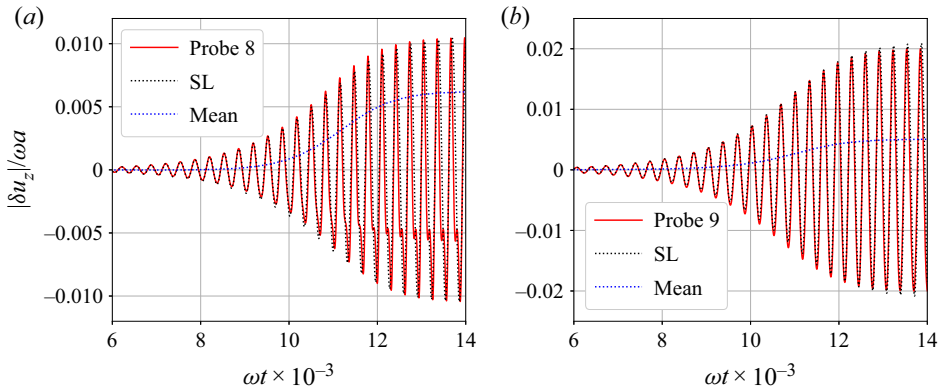
Figure 13. Axial velocity relative to the mean flow ( |\delta u_z| ) at sample probe positions 8 and 9 ( r = 1.5a , z = 0.1h and r = 1.5a , z = 0.25h ). Results from numerical simulations (red) are compared with solutions of the Stuart–Landau (SL) equation (black dots), with \Omega = (19.0 + 0.74i) \times 10^{-3}\omega and \Gamma = (-2.65 + 3.64i) \times 10^{-7}\omega .
