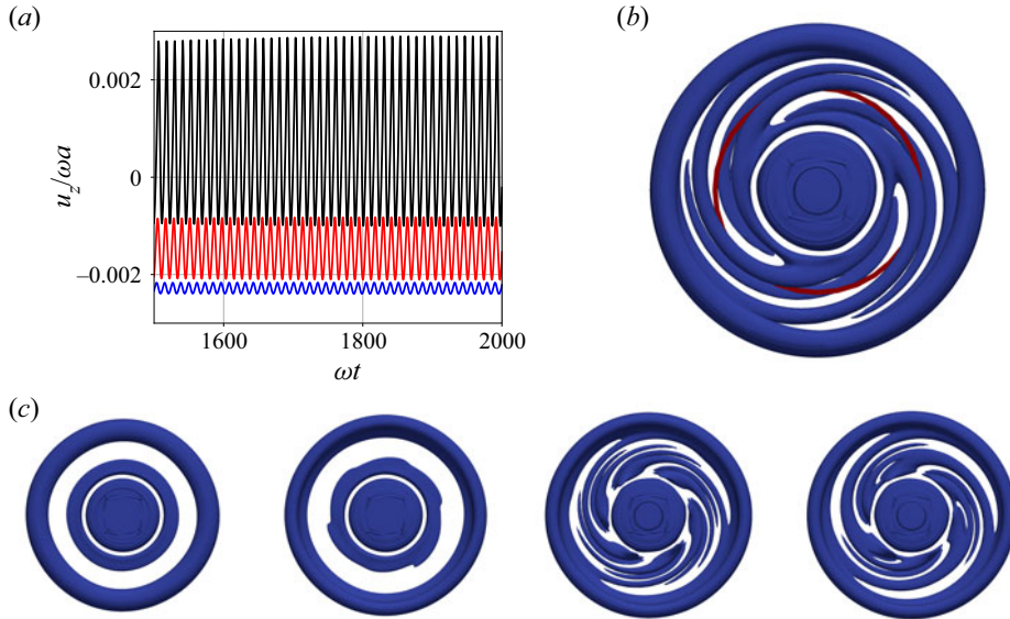
Figure 17. Oscillatory flow at Re = 1200 with the central plane of the rotating disk located at the quarter height z_{disk} = 0.25h . (a) Axial velocity at a single radial position r = 2a , indicated by the red circle. The circle is coplanar with the central plane of the disk ( z = 0.25h ). The three probes are near the base of the container ( z = 0.1h ), coplanar with the disk ( z = 0.25h ) and in the fluid above the disk ( z = 0.45h ). (b) Isosurface of Q = 0.0032\omega^2 at \omega t = 4800 , showing three pairs of spiral vortices. (c) Isosurfaces of Q = 0.0032\omega^2 at \omega t = 120, 240, 360, 480 .
