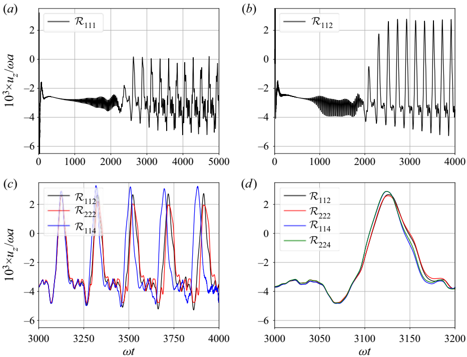
Figure 16. Oscillations of the axial velocity at Re = 1000 for mesh resolutions \mathcal{R}_{111} , \mathcal{R}_{112} , \mathcal{R}_{222} , \mathcal{R}_{114} and \mathcal{R}_{224} . The probe is at r = 2a , z = 0.45h .
