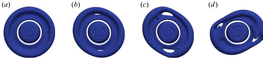
Figure 9. Isosurface of Q = 0.0032\omega^2 at Re = 800 : (a) \omega t = 800 ; (b) \omega t = 3520 ; (c) \omega t = 3840 ; and (d) \omega t = 4800 .
