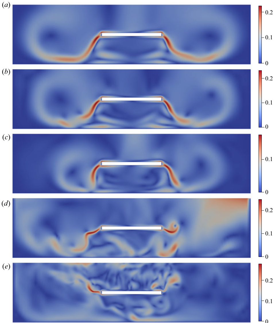
Figure 19. Flow fields at higher Reynolds numbers: (a) Re = 1200 ; (b) Re = 1500 ; (c) Re = 2000 ; (d) Re = 3000 ; (e) Re = 5000 . The colour scale indicates the magnitude of the in-plane flow field, u_{yz} = \sqrt{u_y^2 + u_z^2} .
