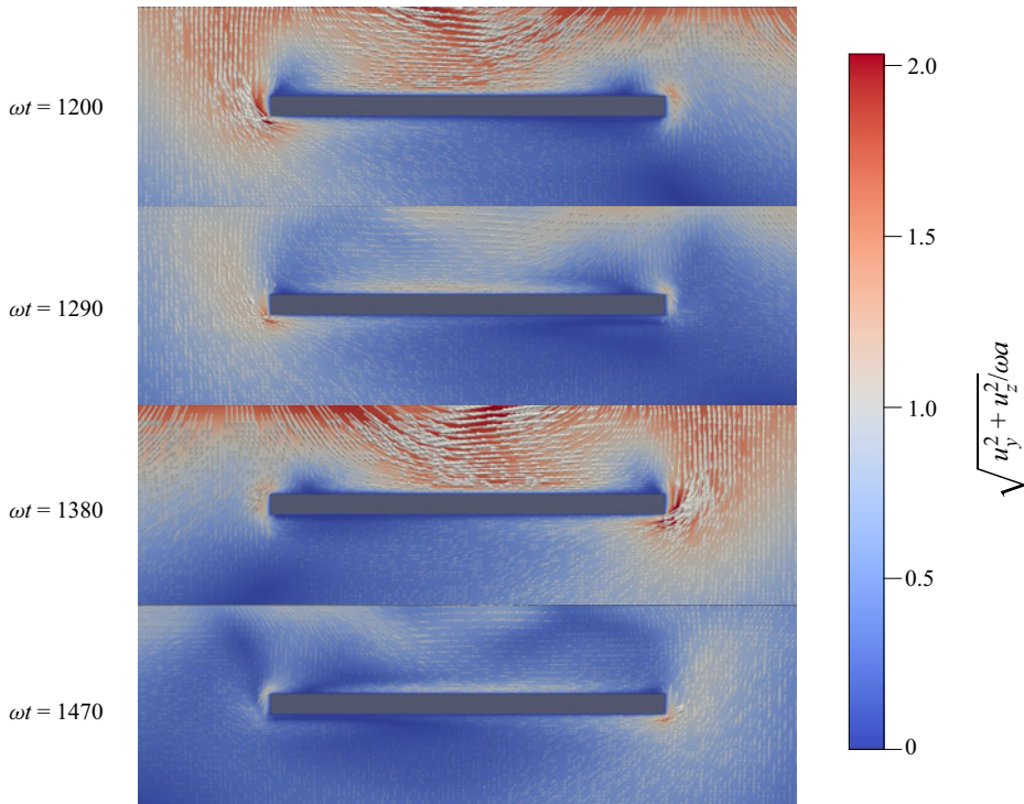
Figure 18. Oscillatory flow at Re = 300 with the central plane of the rotating disk located at the three-quarter height, z_{disk} = 0.75h ; the flow field near the rotating disk is projected on the yz plane. Flow fields are shown at four successive times: (a) \omega t = 1200 ; (b) \omega t = 1290 ; (c) \omega t = 1380 ; and (d) \omega t = 1470 . The colour scale indicates the magnitude of the in-plane flow field, u_{yz} = (u_y^2 + u_z^2)^{1/2} .
