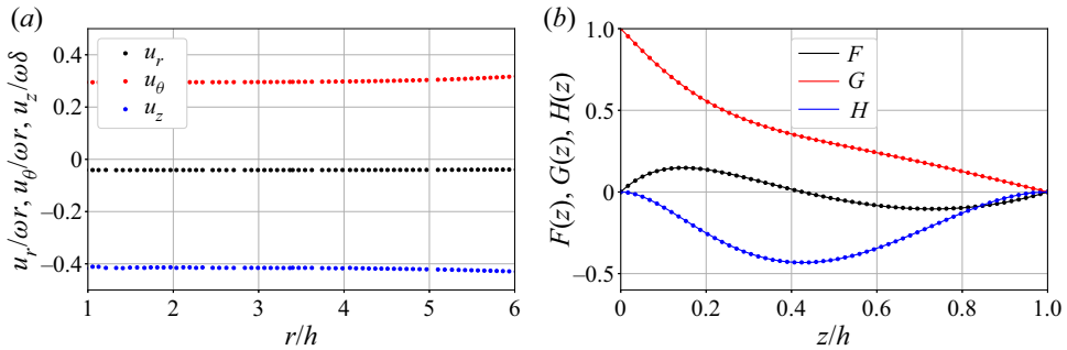
Figure 3. Dimensionless velocity components F(z), G(z), H(z) in a cavity with aspect ratio A = 0.1 and Re_h = 30 . (a) The functions u_r/(\omega r) , u_\theta/(\omega r) and u_z/(\omega \delta) at the midplane position z = 0.5h . There is a window between r = 2h and r = 4h where the solution is smooth and almost independent of r . (b) The functions F(z), G(z), H(z) derived from finite-volume simulations at r = 3h (points) are compared with similarity solutions (solid lines).
