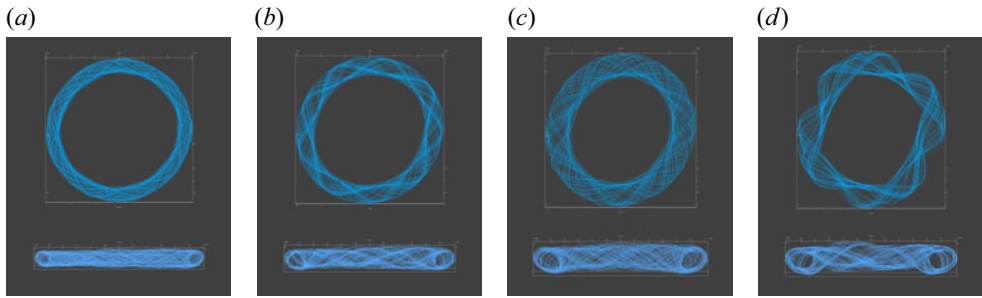
Figure 14. Streamlines showing the outline of the large vortex roll at different times: Re = 700 ; (a) \omega t = 9100 ; (b) \omega t = 9800 ; (c) \omega t = 10150 ; (d) \omega t = 10500 . The upper subpanels show the view from the vertical ( z ) axis, and the lower subpanels the view from the horizontal ( y ) axis.
