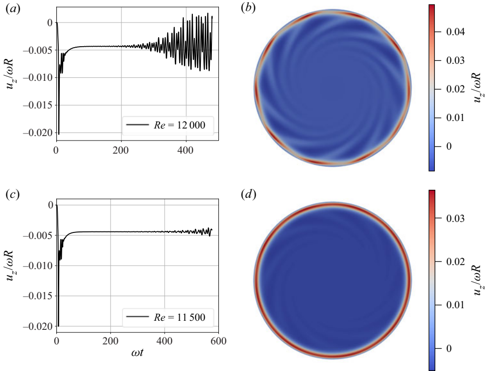
Figure 6. Axial velocity measured by a probe located at r = 4.17h , z = 0.9h , together with a map of the axial velocity in the plane z = 0.9h : (a,b) Re = 12\,000 and (c,d) Re = 11\,500 .
