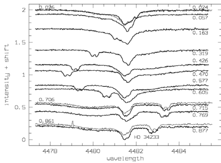
Figure 1. HERMES spectra of DV Cam. Thick lines: spectra taken 2011 Feb. 17-27, thin lines: 2011 Jan. 9-11.
