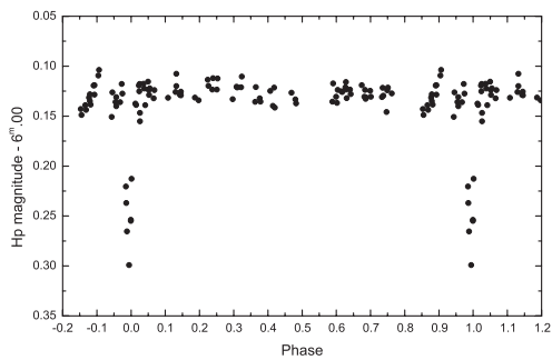
Figure 2. DV Cam light curve phased with ephemeris Pri HJD=2448751.926 + 6.67840 × E.
