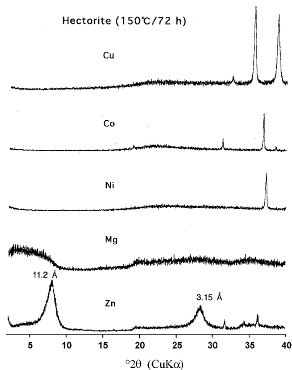
Figure 5. XRD patterns of synthetic products prepared by reacting \text{SiO}_2 with ZnO, MgO, NiO, CoO and CuO.
