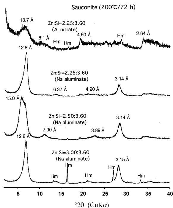
Figure 2. XRD patterns of synthetic saunonites prepared with different Zn/Si ratios and different precursors. HM = hemimorphite.
