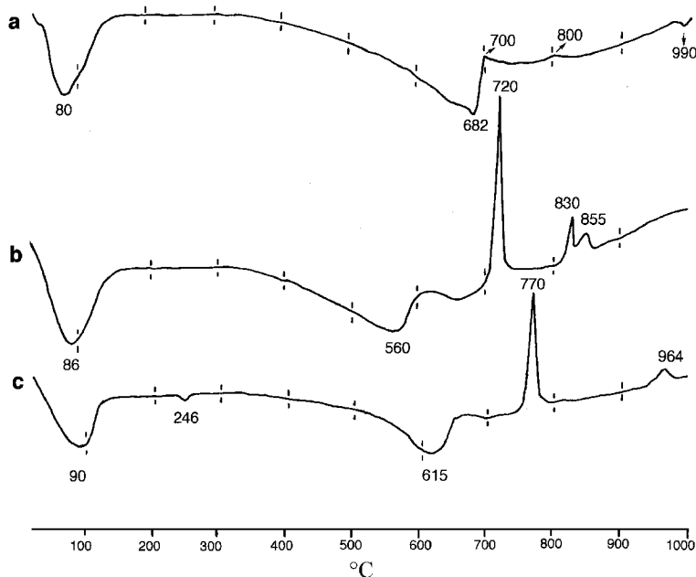
Figure 7. DTA curves of different synthetic smectites: (a) hectorite, (b) sauconite, and (c) Zn-hectorite (samples are the same as in Table 5).
