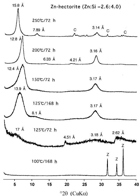
Figure 3. XRD patterns of synthetic Zn-hectorites prepared at different temperatures. C = cristobalite; Z = ZnO.
