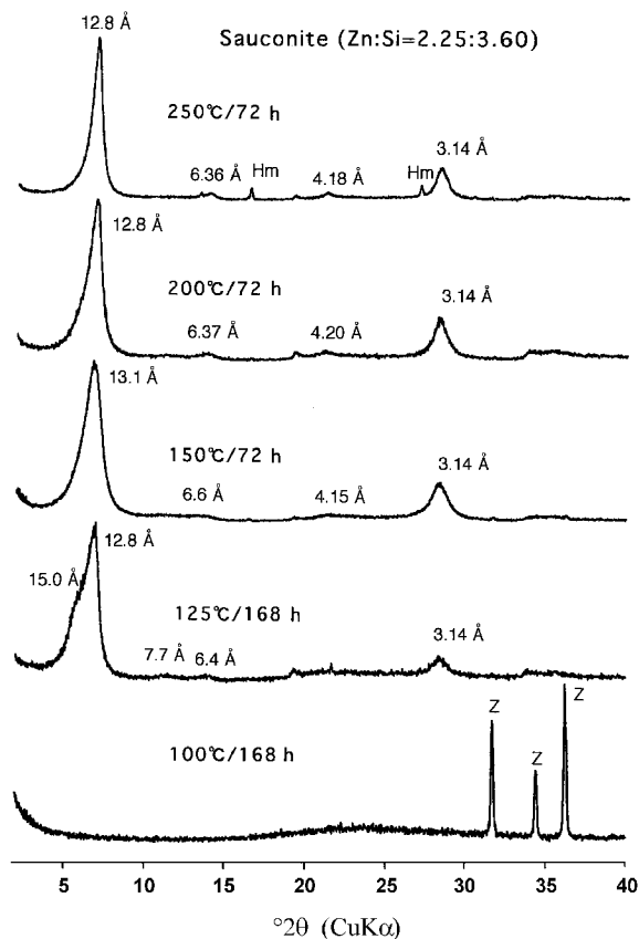
Figure 1. XRD patterns of synthetic saucunites prepared at different temperatures. HM = hemimorphite; Z = ZnO.
