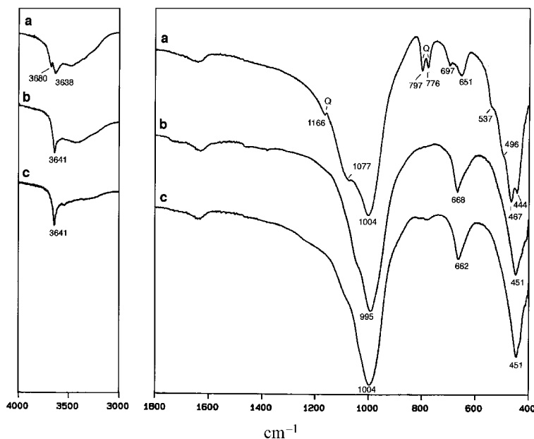
Figure 6. IR spectra of different synthetic smectites: (a) hectorite, (b) sauconite, and (c) Zn-hectorite (samples are the same as in Table 5).
