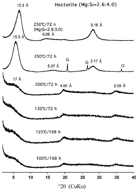
Figure 4. XRD patterns of synthetic hectorites prepared at different temperatures. Q = Quartz.
