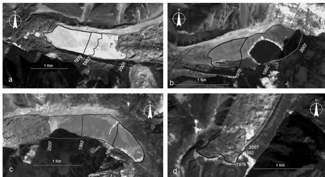
Fig. 2. Examples of glacier retreat and lake expansion from the Dudh Koshi basin: (a) Imja Glacier and Tsho; (b) glacier 262 (lake 464) in Hungu valley; (c) Lumding Glacier and Tsho; (d) Khumbu Glacier.
