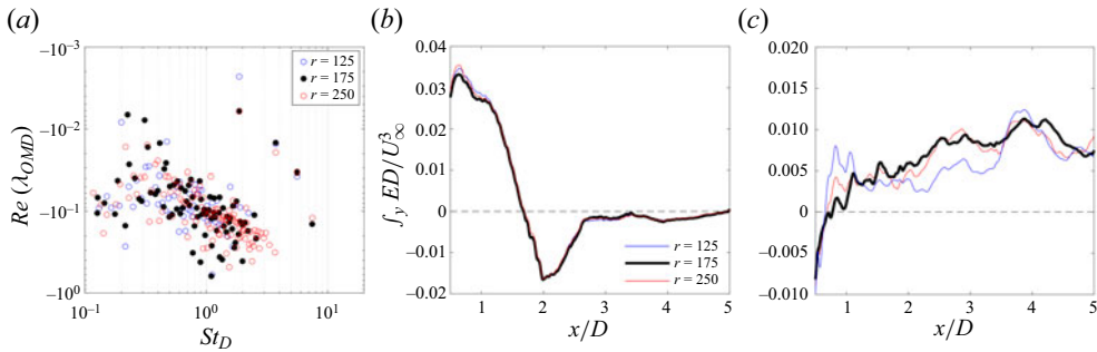
Figure 18. (a) The OMD spectra for different ranks r . Plots (b,c) shows the streamwise evolution of the spanwise-averaged \tilde{P}_l term for f_r and f_{vm} , respectively, for different r .
