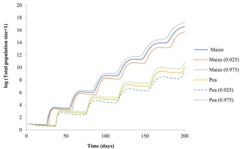
Figure 5. Total population size of the Spodoptera frugiperda projected by using life tables of 0.975 and 0.025 percentiles of intrinsic rate on increase ( r ) on maize and pea with an initial population of ten eggs.
