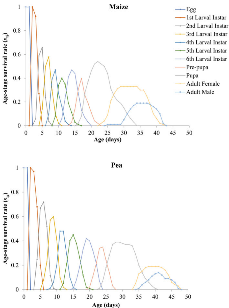
Figure 1. Age-stage-specific survival rate ( s_{xj} ) of the Spodoptera frugiperda reared on maize and pea.
