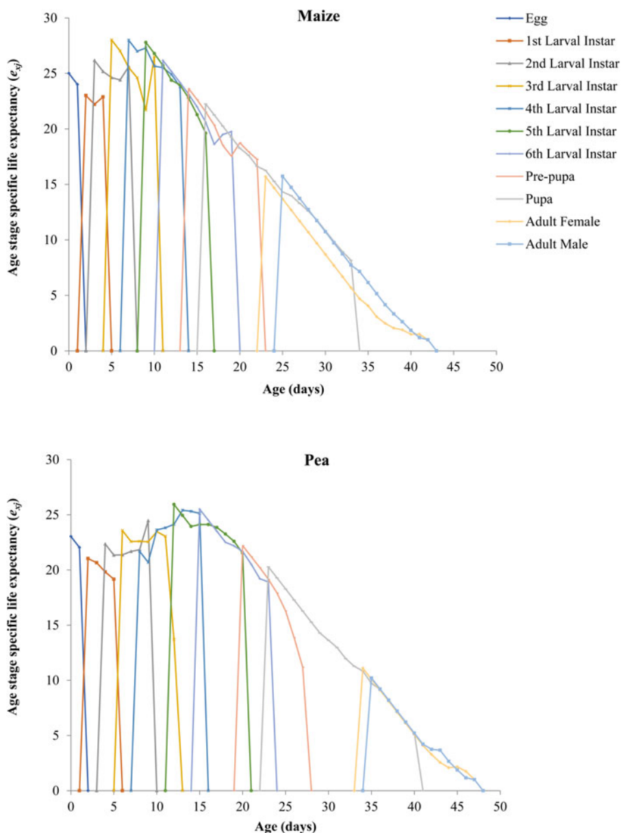
Figure 3. Age-stage-specific life expectancy ( e_{sj} ) of the Spodoptera frugiperda reared on maize and pea.
