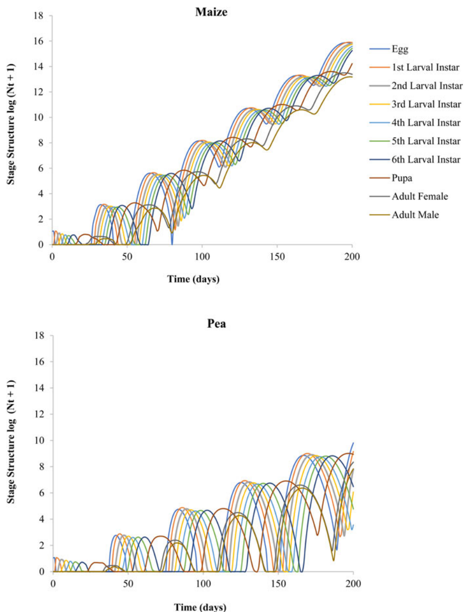
Figure 6. Population projection of Spodoptera frugiperda reared on maize and pea with an initial population of ten eggs.
