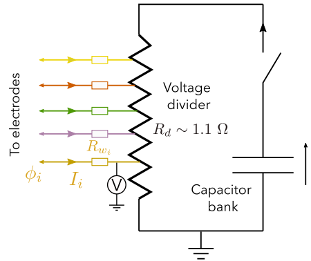
FIGURE 1. Picture of the multidisk electrode used in this experimental campaign (a) and electric circuit used to bias each electrode (b). The outer radius of each electrode is r_i = 2.54i cm, i \in \llbracket 1, 5 \rrbracket . Here R_{w_i} is the resistance of the cable between the point of measure near the voltage divider and the disk \mathcal{E}_i in the machine.
