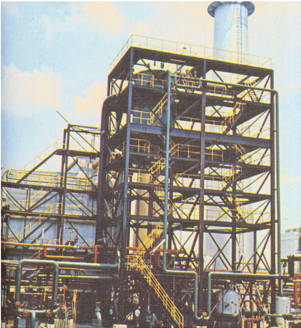
Figure 6. A large industrial boiler manufactured and installed by TMMC for Chinese Petroleum Corp. in Kaohsiung in 1971. This boiler has a capacity of producing steam at a rate of 240,000 lbs per hour. Taiji yuekan 8.5 (Oct, 1971), cover.
