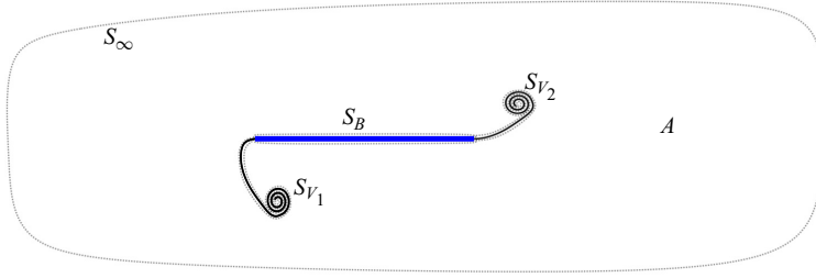
Figure 7. Contours and areal region used in Appendix A.2 to calculate the aerodynamic force on a flat plate that is translating and rotating in a fluid. The flat plate is coloured blue, the vortex sheets from the leading and trailing edges are solid black lines, whereas the contours used in the integrations are dotted black lines.
