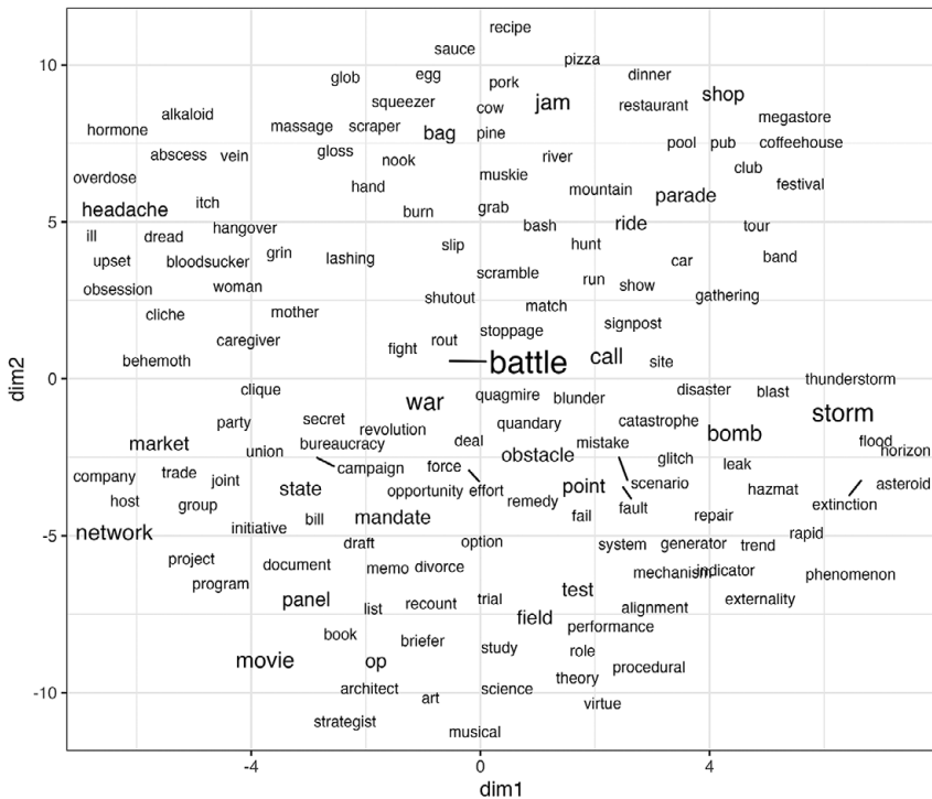
Figure 2 Semantic vector-space analysis of the lemmas occurring in [ the mother of all X ] in ENCOW.
