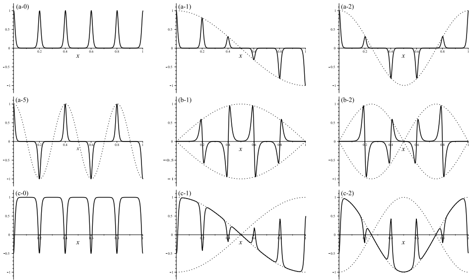
Figure 3. Profiles of eigenfunctions for (LP - ) with u_{10,\varepsilon}^-(x) ; (a-0) \varphi_0^- , (a-1) \varphi_1^- , (a-2) \varphi_2^- , (a-5) \varphi_5^- , (b-1) \varphi_6^- , (b-2) \varphi_7^- , (c-0) \varphi_{10}^- , (c-1) \varphi_{11}^- and (c-2) \varphi_{12}^- .
