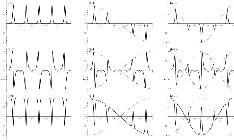
Figure 2. Profiles of eigenfunctions for (LP + ) with u_{10,\varepsilon}^+(x) ; (a-0) \varphi_0^+ , (a-1) \varphi_1^+ , (a-2) \varphi_2^+ , (b-0) \varphi_5^+ , (b-1) \varphi_6^+ , (b-2) \varphi_7^+ , (c-0) \varphi_{10}^+ , (c-1) \varphi_{11}^+ and (c-2) \varphi_{12}^+ .
