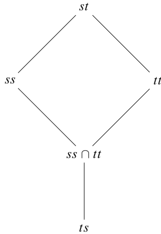
Figure 2. The five intersective mixed consequence relations.
