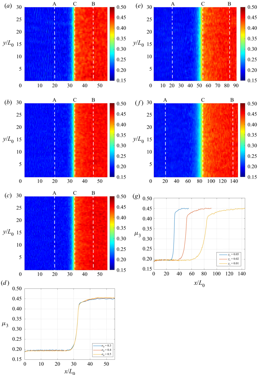
Figure 6. Mean skewness of surface elevation \eta for uneven bottoms at different directional spreads \sigma_\theta and slope angles \gamma_s with initial BFI = 0.4 (blue, \sigma_\theta = 0.3 ; red, \sigma_\theta = 0.4 ; yellow, \sigma_\theta = 0.5 ; g: blue, \gamma_s = 0.05 ; red, \gamma_s = 0.02 ; yellow, \gamma_s = 0.01 ). (a) \sigma_\theta = 0.3 , \gamma_s = 0.05 , (b) \sigma_\theta = 0.4 , \gamma_s = 0.05 , (c) \sigma_\theta = 0.5 , \gamma_s = 0.05 , (d) \sigma_\theta = 0.3, 0.4, 0.5 , \gamma_s = 0.05 , (e) \sigma_\theta = 0.3 , \gamma_s = 0.02 , (f) \sigma_\theta = 0.3 , \gamma_s = 0.01 and (g) \sigma_\theta = 0.3 , \gamma_s = 0.05, 0.02, 0.01 .
