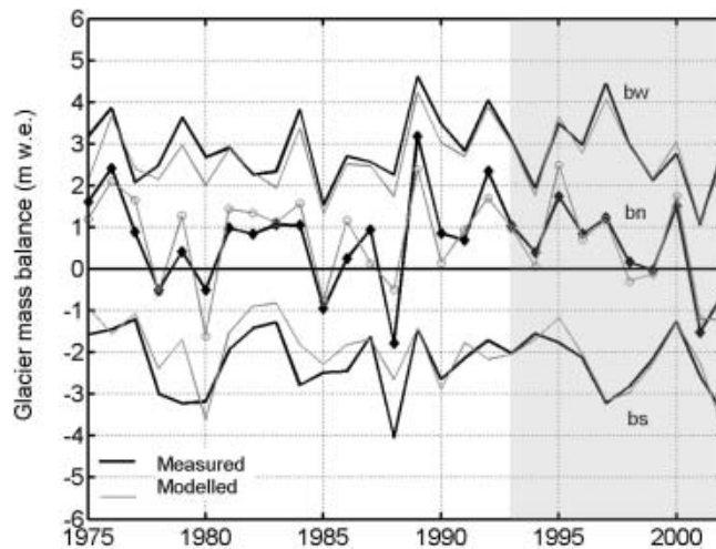
Fig. 5. The temporal evolution of mass balance of Engabreen. Values of winter ( b_w ), summer ( b_s ) and net ( b_n ) mass balances are shown separately. The shaded area indicates the calibration period.
