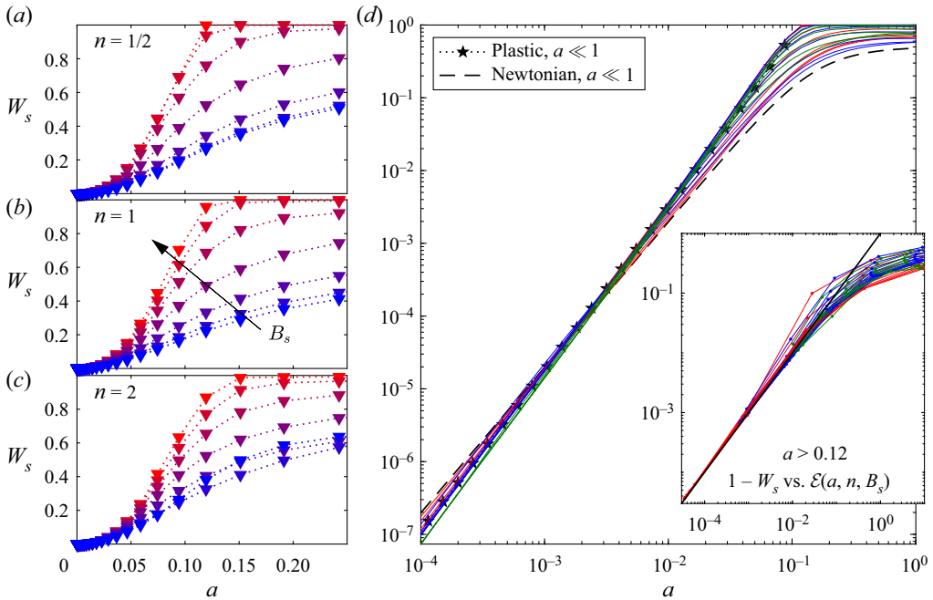
Figure 3. Locomotion speed W_s against wave amplitude a for a swimmer driven by sinusoidal waves in Herschel–Bulkeley fluid with (a) n = \frac{1}{2} , (b) n = 1 and (c) n = 2 . Examples with B_s = 10^{-3}, 10^{-1}, \dots, 10^3 are presented (colour coded by B_s , from blue to red). The data are replotted logarithmically over a wider range of a in (d), with n = \frac{1}{2}, 1 and 2 shown in red, blue and green (respectively). The dashed line shows the result for Newtonian fluid (§ 3.1; (3.2)), and the low-amplitude, plastic solutions of § 3.2 are shown by the stars. The inset in (d) shows the data for a > 0.12 , replotted as 1 - W_s against the quantity \mathcal{E}(a, n, B_s) defined in (3.17a,b); the solid (black) line shows the prediction 1 - W_s = \mathcal{E} from § 3.3.
