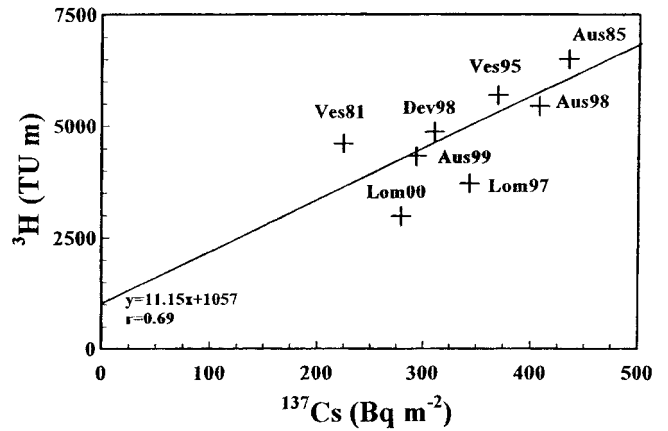
Fig. 9. ^3\text{H} vs ^{137}\text{Cs} fall-out from atmospheric nuclear tests at eight Arctic ice-core locations.
