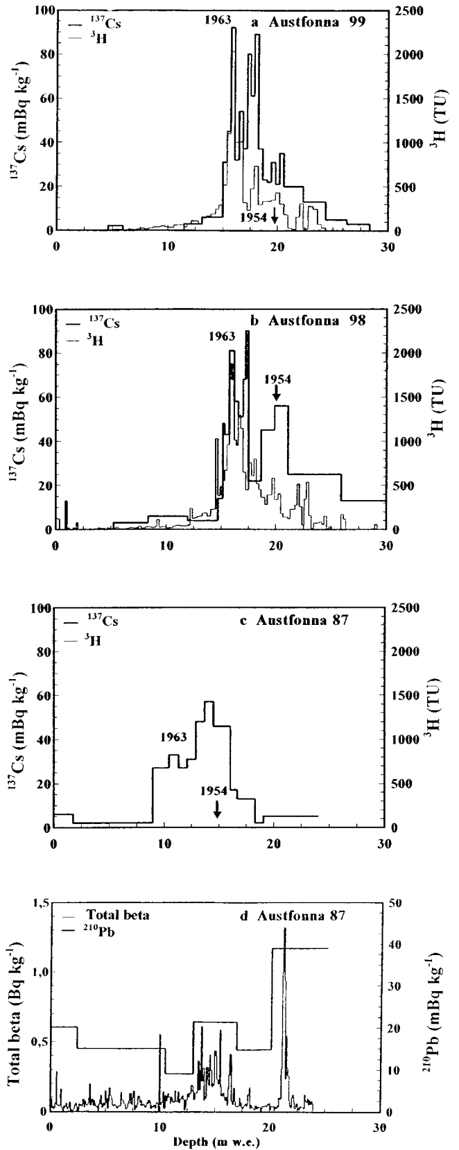
Fig. 4. Radioactivity at time of fall-out ( ^{137}\text{Cs} and ^3\text{H} ), and at time of measurement (total beta and ^{210}\text{Pb} , respectively, 1988 and 1993) vs depth for three ice cores from Austfonna (a–d). The arrow indicates the equivalent 1954 computed year.
