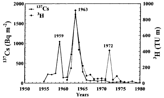
Fig. 2. 137 Cs fall-out at Tromsø and 3 H content in fall-out at Isfjord Radio from atmospheric nuclear tests.
