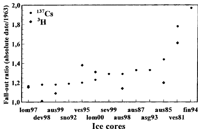
Fig. 7. ^{137}\text{Cs} and ^3\text{H} fall-out ratio from atmospheric nuclear tests, determined from 1963 mean time of fall-out and absolute date of snow layers, respectively.
