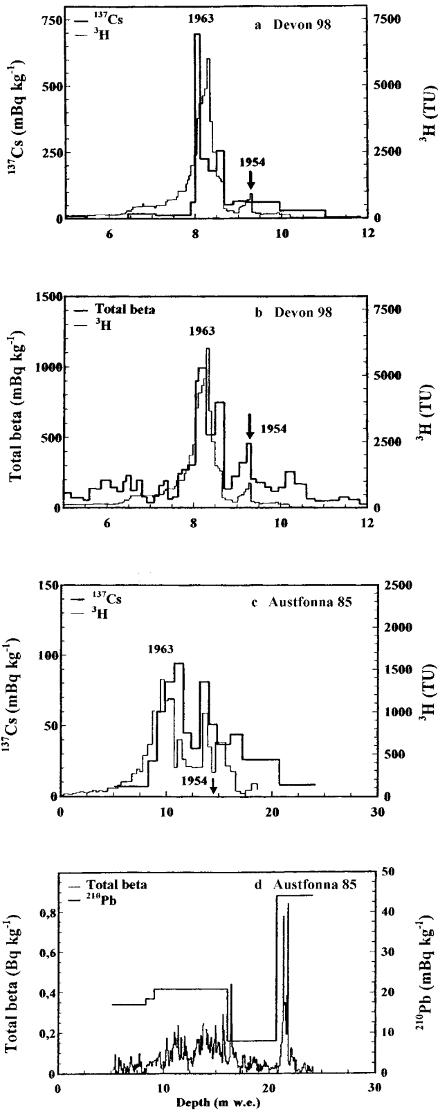
Fig. 3. Radioactivity at time of fall-out ( ^{137}\text{Cs} and ^3\text{H} ), and at time of measurement (total beta and ^{210}\text{Pb} , respectively, 1986 and 1993) vs depth for Devon Ice Cap (a, b) and Austfonna (c, d). ^3\text{H} measurements from Devon Island (thin line) are not continuous. The arrow indicates the equivalent 1954 computed year.
