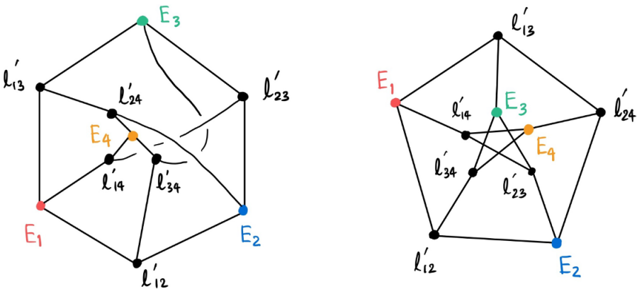
Figure 6.2. The dual graph of the blowup shown in Figure 6.1 is drawn on the left, and it is equivalent to the Petersen graph shown on the right.
