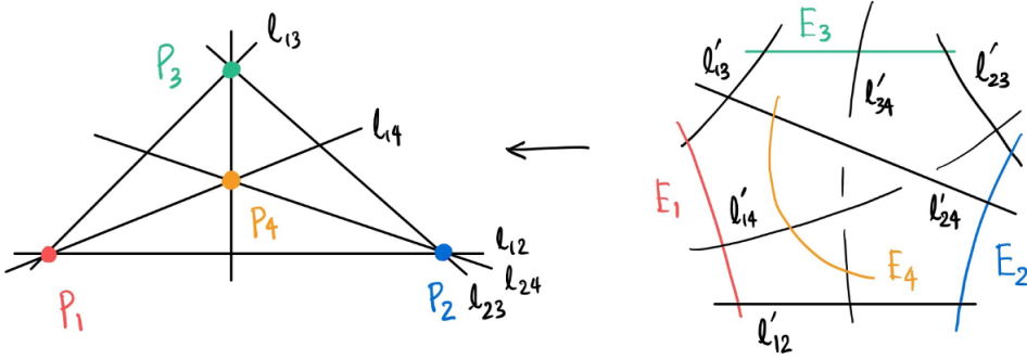
Figure 6.1. Blowing up once at each point p_1, \dots, p_4 results in the diagram above.
