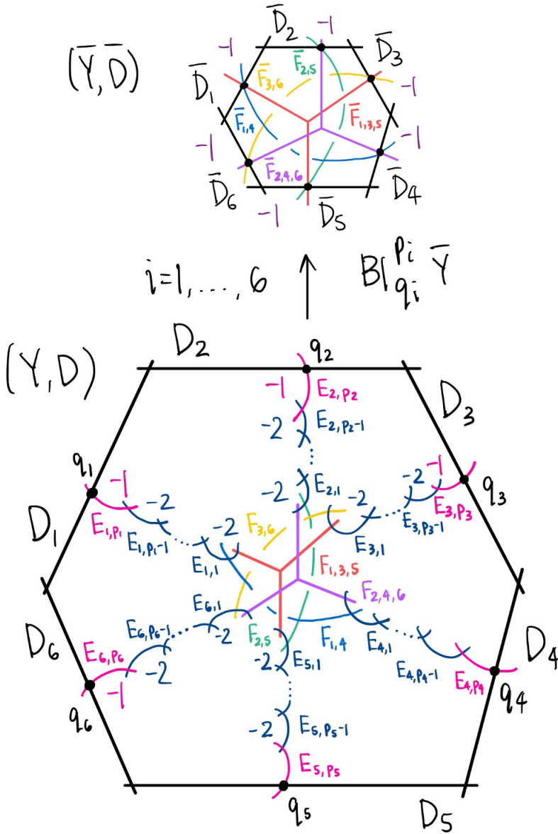
Figure 6.4. This diagram shows the surface (\bar{Y}, \bar{D}) blown up at points q_i , each a total of p_i times, for when n = 6 .
