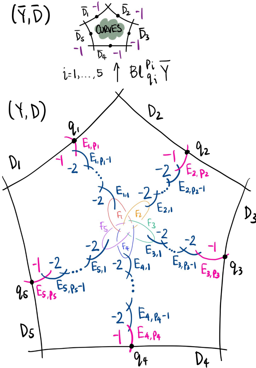
Figure 6.3. Blowing up once at each point q_1, \dots, q_5 results in the diagram above.
