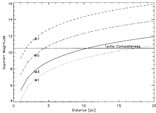
Figure 1. Change of observed magnitude with distance under the assumption of negligible absorption. The straight line indicates the approximate completeness limit of the Tycho catalogue.
