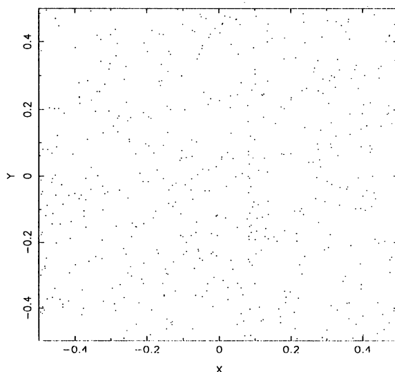
Figure 1. A computer generated distribution of galaxies produced in the QSSC for the case P/Q = 20 , within 5 cycles, for the fraction x = 0.3 . Filamentary structure separated by voids is evident. (Picture generated by A. Nayari).
