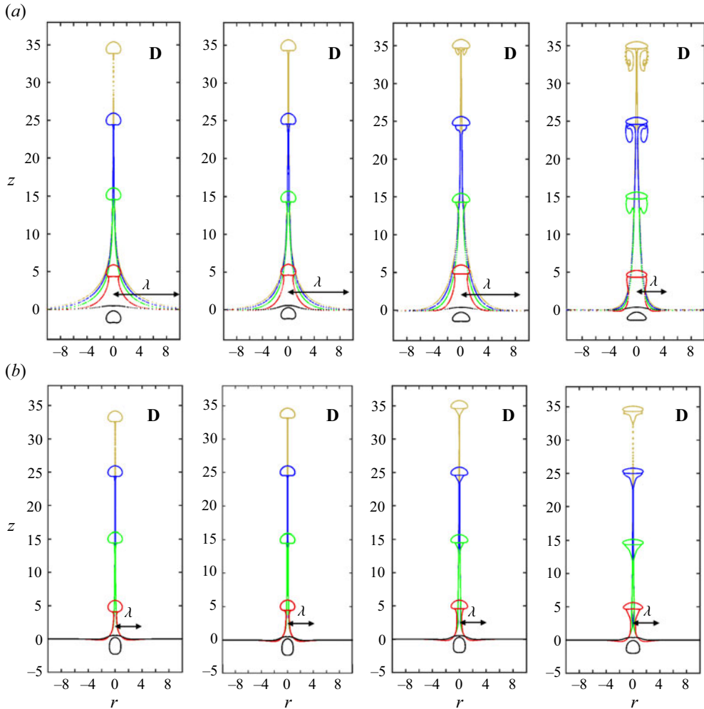
Figure 8. Effect of increasing Ar on the entrainment at moderate Bo : Bo = 5 and \rho = 1 , m = 1 for (a) Y = 0 and (b) Y = 0.1 ; from left to right Ar = 5, 10, 50 and 500 . For colours refer to the caption of figure 5.
